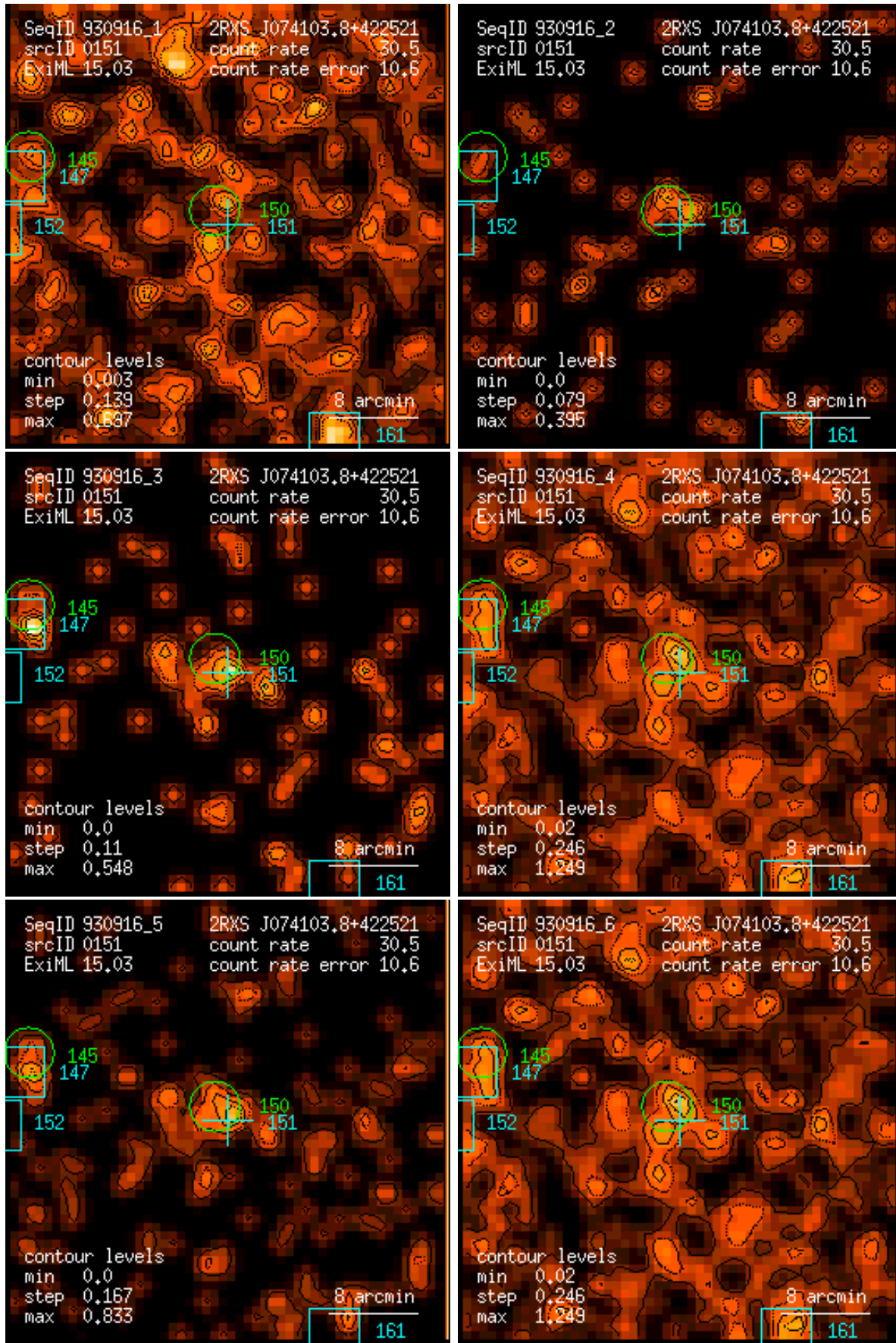
Figure 151: RASS 930916: detection 0151: band rate images, Gaussian filter: (1) PSPC channels 11 – 41, (2) 52 – 90, (3) 91 – 201, (4) 11 – 235, (5) 52 – 201, (6) 11 – 201. Broad band rates in counts/ks. Band rate contour levels in counts/ks/arcmin 2 .
