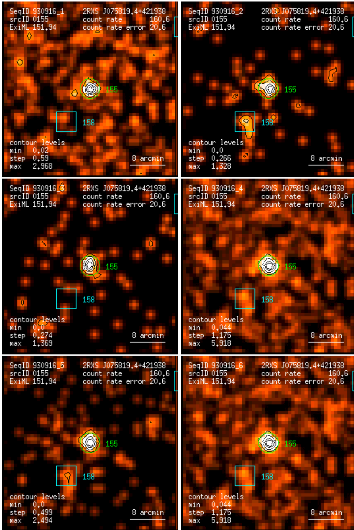
Figure 155: RASS 930916: detection 0155: band rate images, Gaussian filter: (1) PSPC channels 11 – 41, (2) 52 – 90, (3) 91 – 201, (4) 11 – 235, (5) 52 – 201, (6) 11 – 201. Broad band rates in counts/ks. Band rate contour levels in counts/ks/arcmin 2 .
