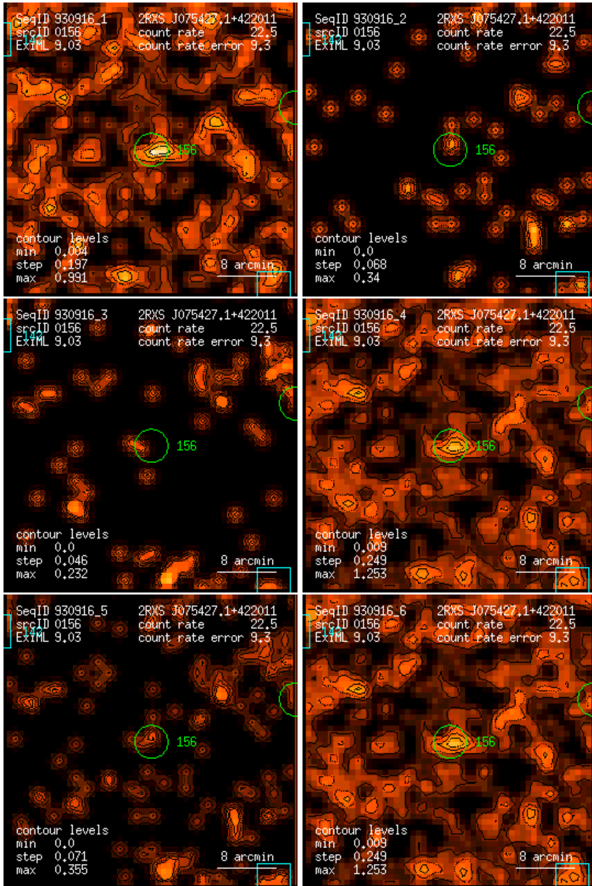
Figure 156: RASS 930916: detection 0156: band rate images, Gaussian filter: (1) PSPC channels 11 – 41, (2) 52 – 90, (3) 91 – 201, (4) 11 – 235, (5) 52 – 201, (6) 11 – 201. Broad band rates in counts/ks. Band rate contour levels in counts/ks/arcmin 2 .
