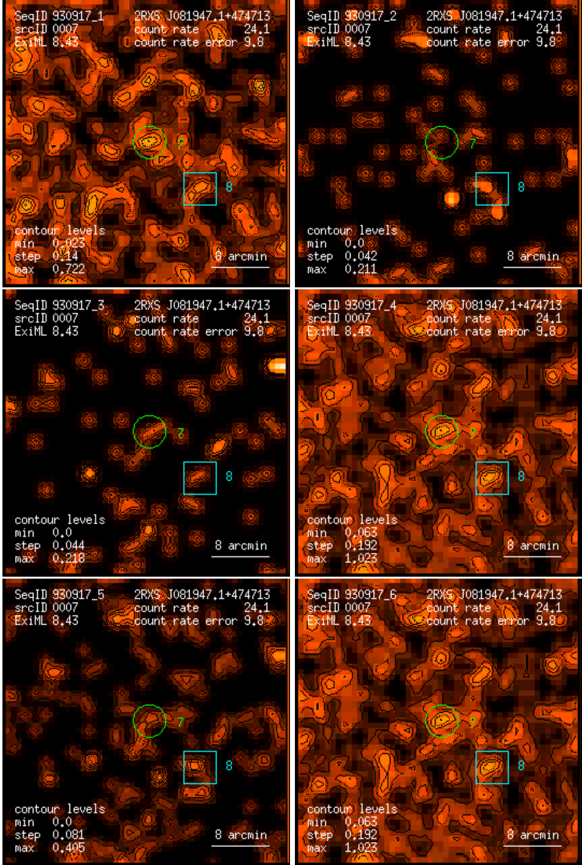
Figure 7: RASS 930917: detection 0007: band rate images, Gaussian filter: (1) PSPC channels 11 – 41, (2) 52 – 90, (3) 91 – 201, (4) 11 – 235, (5) 52 – 201, (6) 11 – 201. Broad band rates in counts/ks. Band rate contour levels in counts/ks/arcmin 2 .
