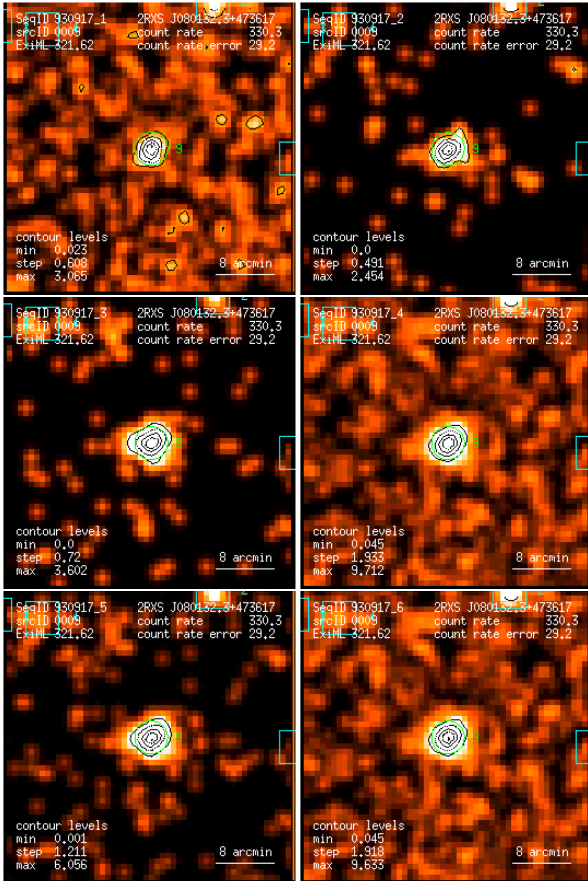
Figure 9: RASS 930917: detection 0009: band rate images, Gaussian filter: (1) PSPC channels 11 – 41, (2) 52 – 90, (3) 91 – 201, (4) 11 – 235, (5) 52 – 201, (6) 11 – 201. Broad band rates in counts/ks. Band rate contour levels in counts/ks/arcmin 2 .
