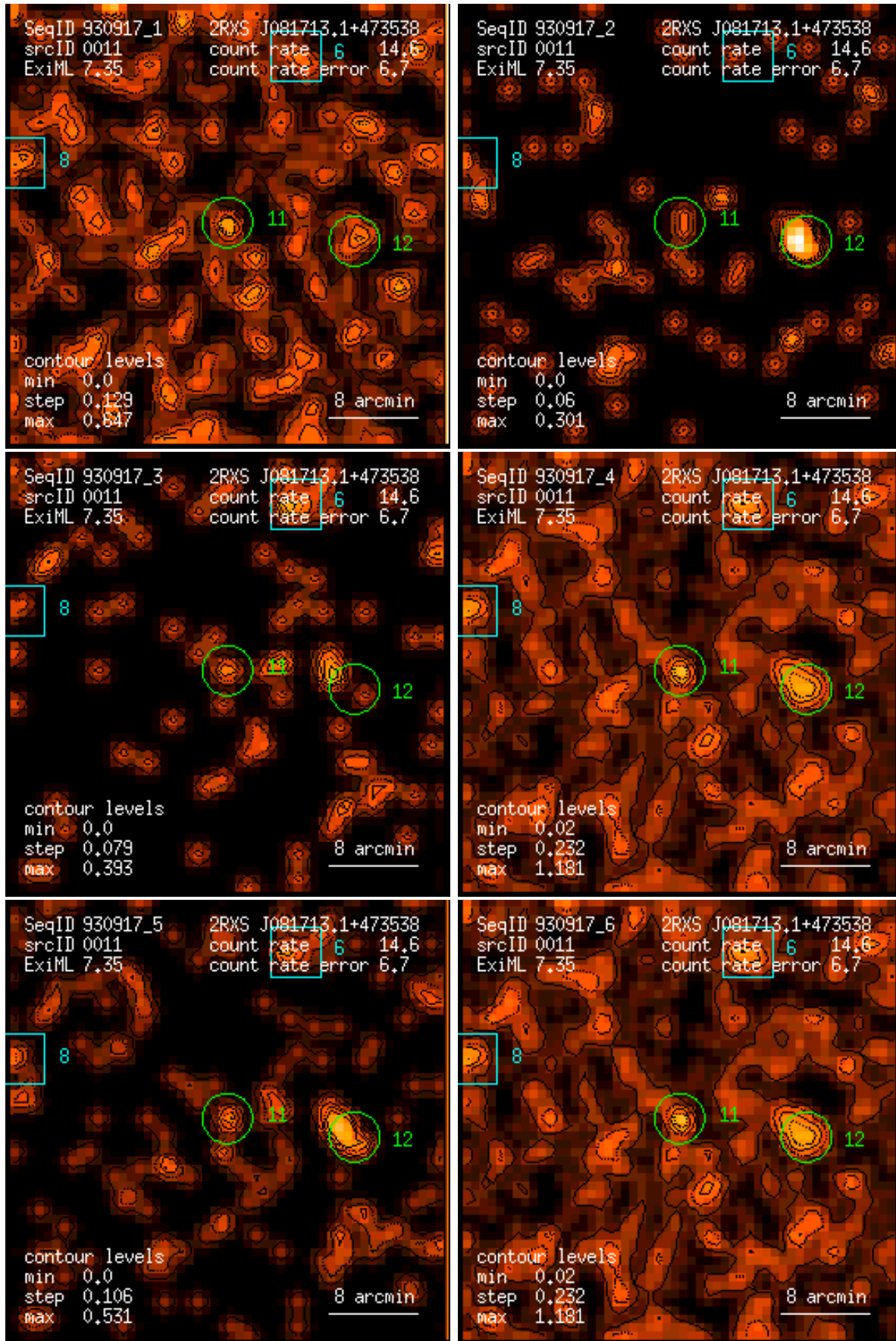
Figure 11: RASS 930917: detection 0011: band rate images, Gaussian filter: (1) PSPC channels 11 – 41, (2) 52 – 90, (3) 91 – 201, (4) 11 – 235, (5) 52 – 201, (6) 11 – 201. Broad band rates in counts/ks. Band rate contour levels in counts/ks/arcmin 2 .
