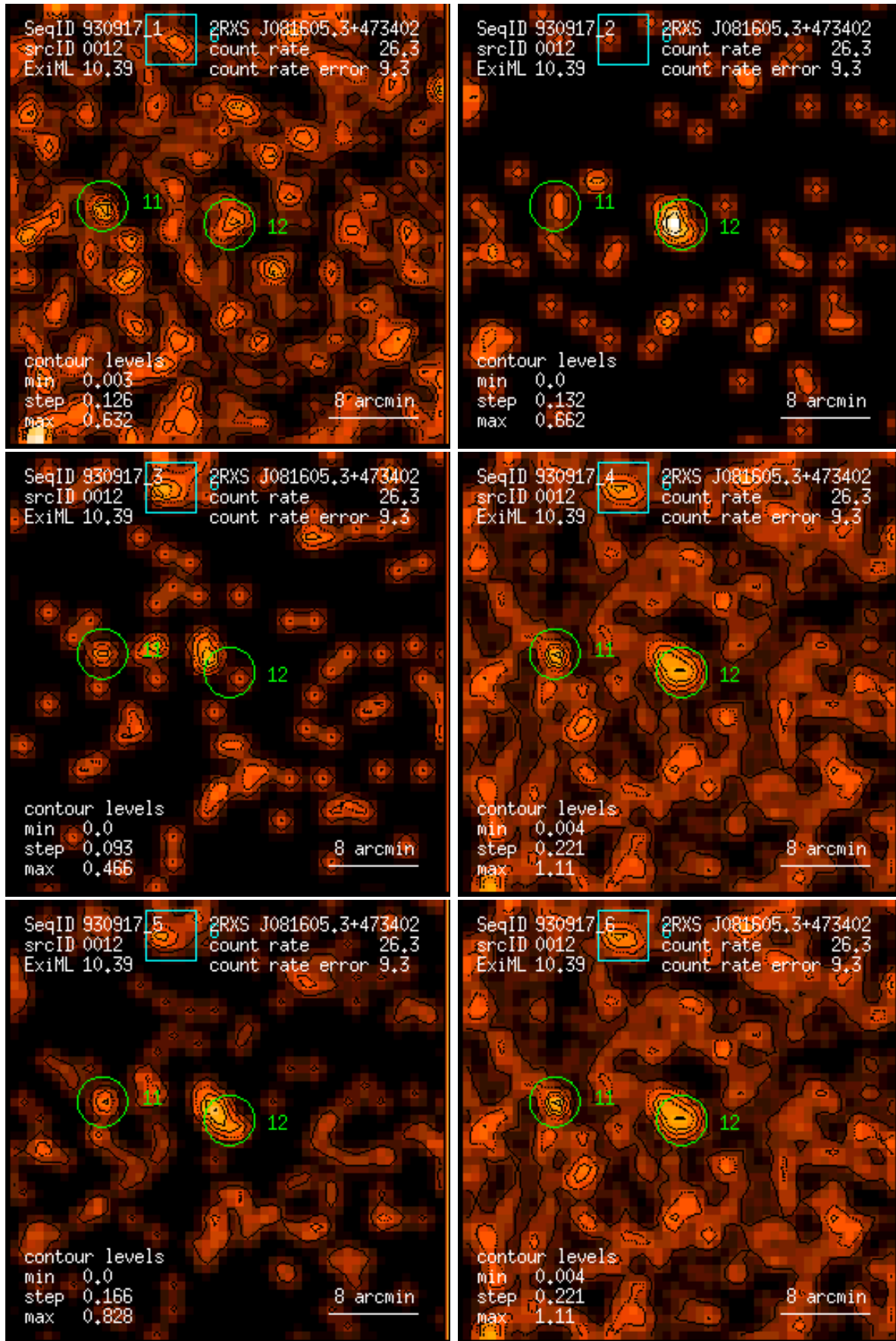
Figure 12: RASS 930917: detection 0012: band rate images, Gaussian filter: (1) PSPC channels 11 – 41, (2) 52 – 90, (3) 91 – 201, (4) 11 – 235, (5) 52 – 201, (6) 11 – 201. Broad band rates in counts/ks. Band rate contour levels in counts/ks/arcmin 2 .
