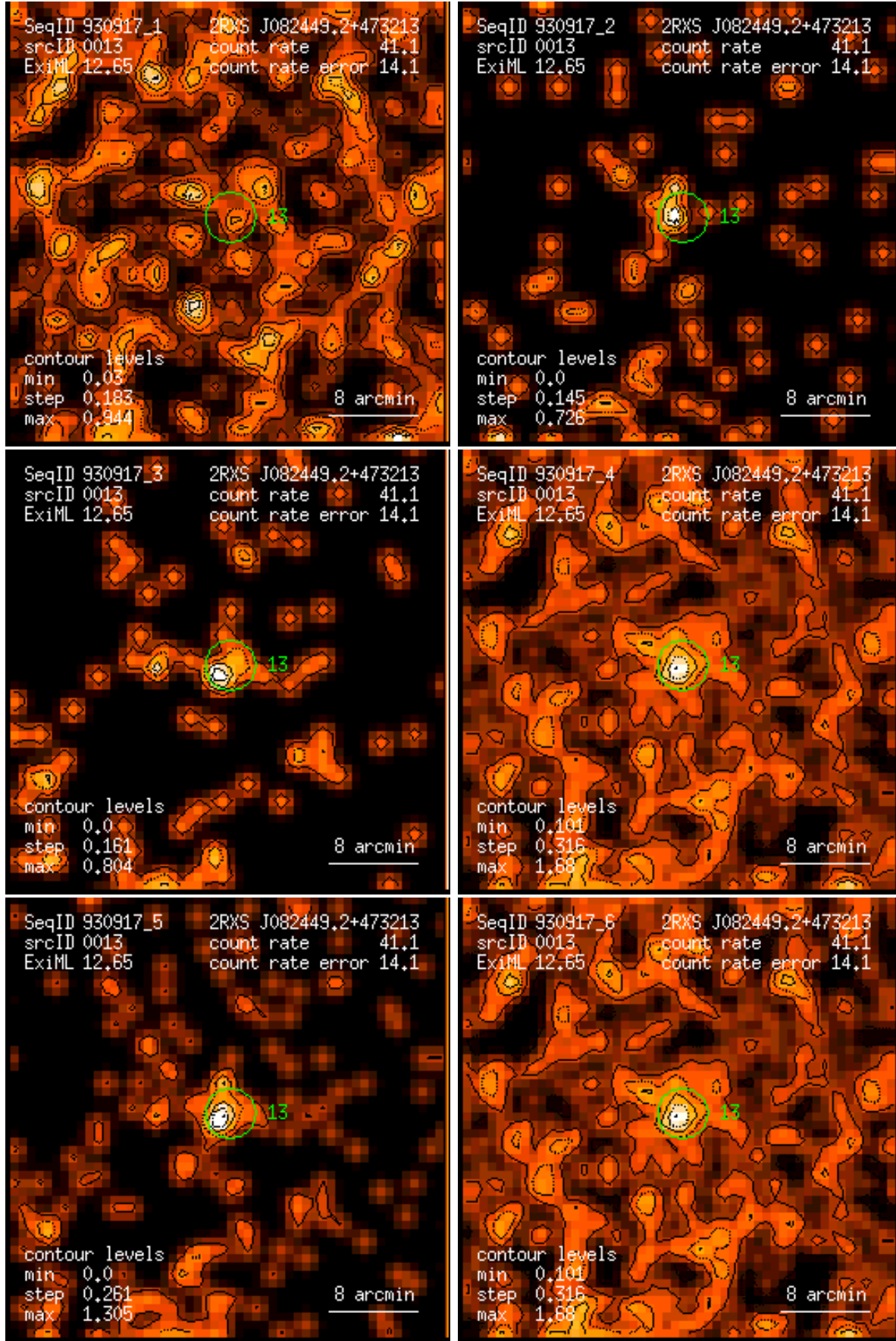
Figure 13: RASS 930917: detection 0013: band rate images, Gaussian filter: (1) PSPC channels 11 – 41, (2) 52 – 90, (3) 91 – 201, (4) 11 – 235, (5) 52 – 201, (6) 11 – 201. Broad band rates in counts/ks. Band rate contour levels in counts/ks/arcmin 2 .
