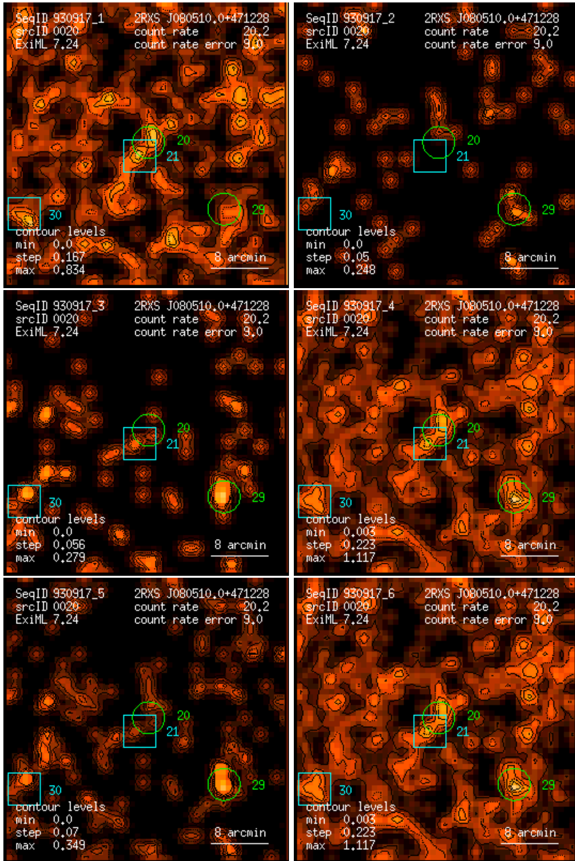
Figure 20: RASS 930917: detection 0020: band rate images, Gaussian filter: (1) PSPC channels 11 – 41, (2) 52 – 90, (3) 91 – 201, (4) 11 – 235, (5) 52 – 201, (6) 11 – 201. Broad band rates in counts/ks. Band rate contour levels in counts/ks/arcmin 2 .
