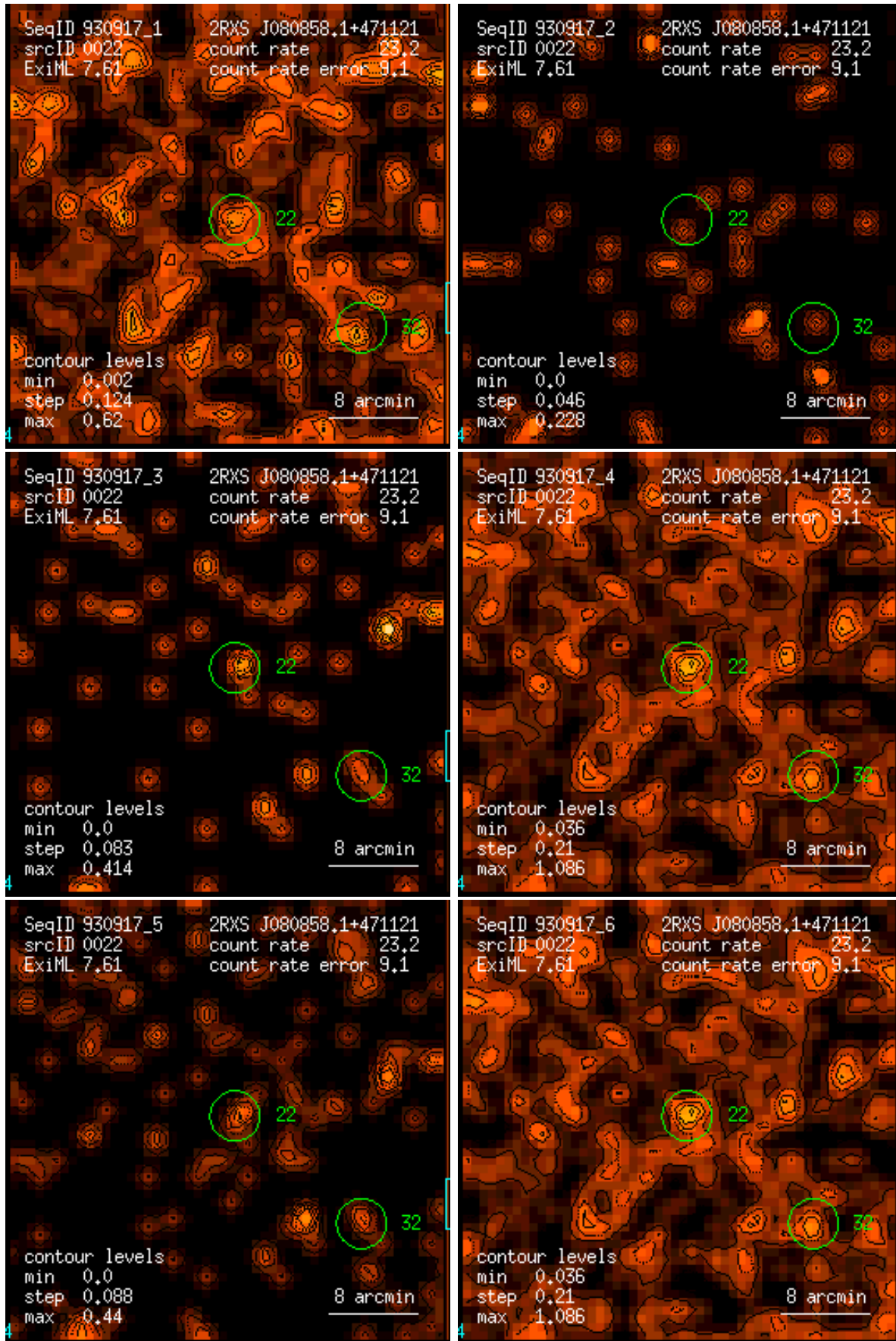
Figure 22: RASS 930917: detection 0022: band rate images, Gaussian filter: (1) PSPC channels 11 – 41, (2) 52 – 90, (3) 91 – 201, (4) 11 – 235, (5) 52 – 201, (6) 11 – 201. Broad band rates in counts/ks. Band rate contour levels in counts/ks/arcmin 2 .
