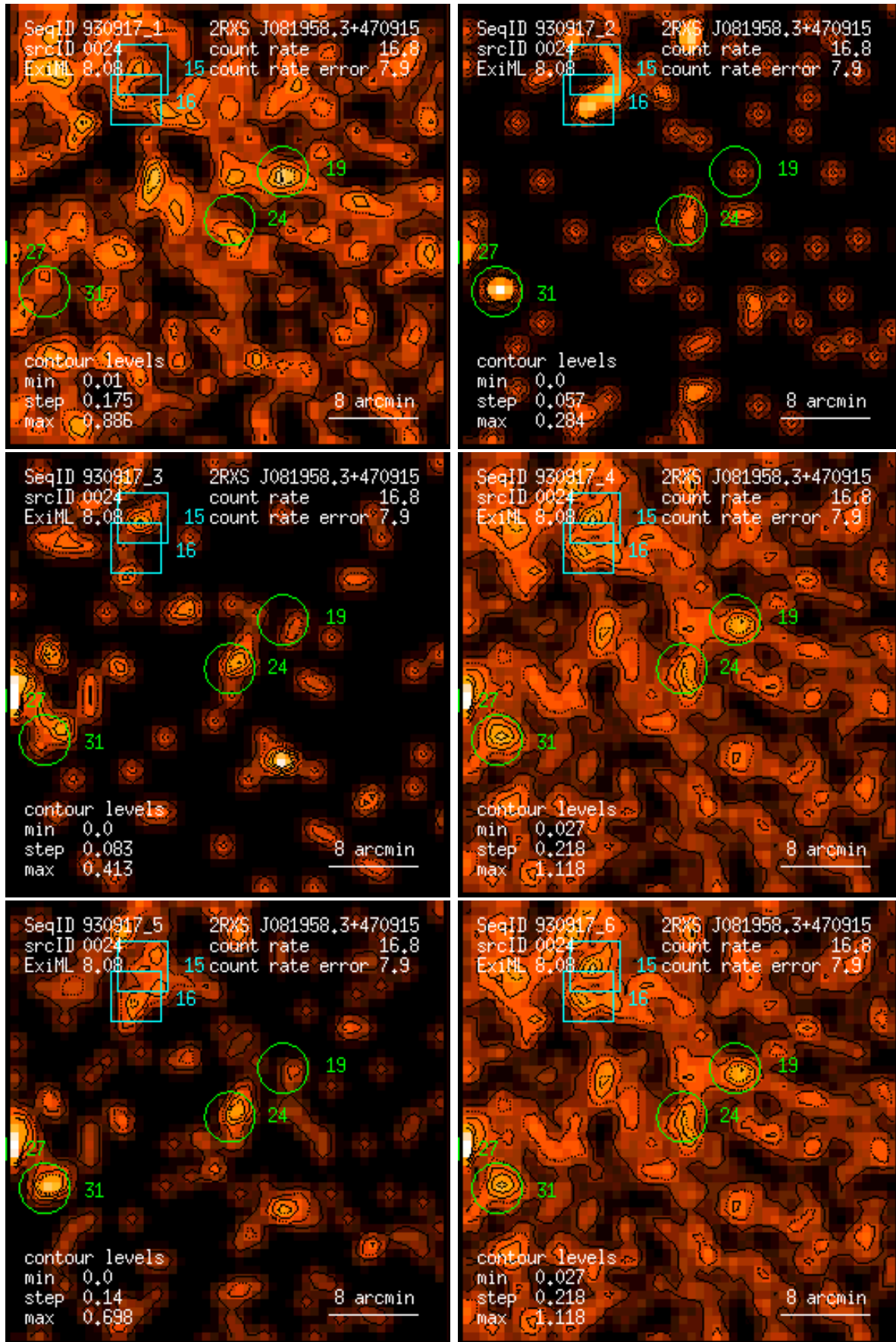
Figure 24: RASS 930917: detection 0024: band rate images, Gaussian filter: (1) PSPC channels 11 – 41, (2) 52 – 90, (3) 91 – 201, (4) 11 – 235, (5) 52 – 201, (6) 11 – 201. Broad band rates in counts/ks. Band rate contour levels in counts/ks/arcmin 2 .
