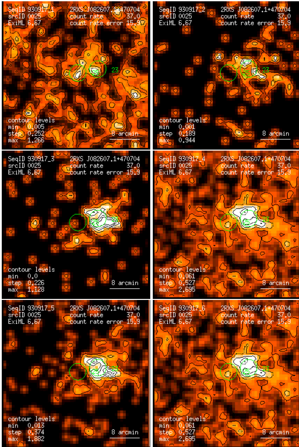
Figure 25: RASS 930917: detection 0025: band rate images, Gaussian filter: (1) PSPC channels 11 – 41, (2) 52 – 90, (3) 91 – 201, (4) 11 – 235, (5) 52 – 201, (6) 11 – 201. Broad band rates in counts/ks. Band rate contour levels in counts/ks/arcmin 2 .
