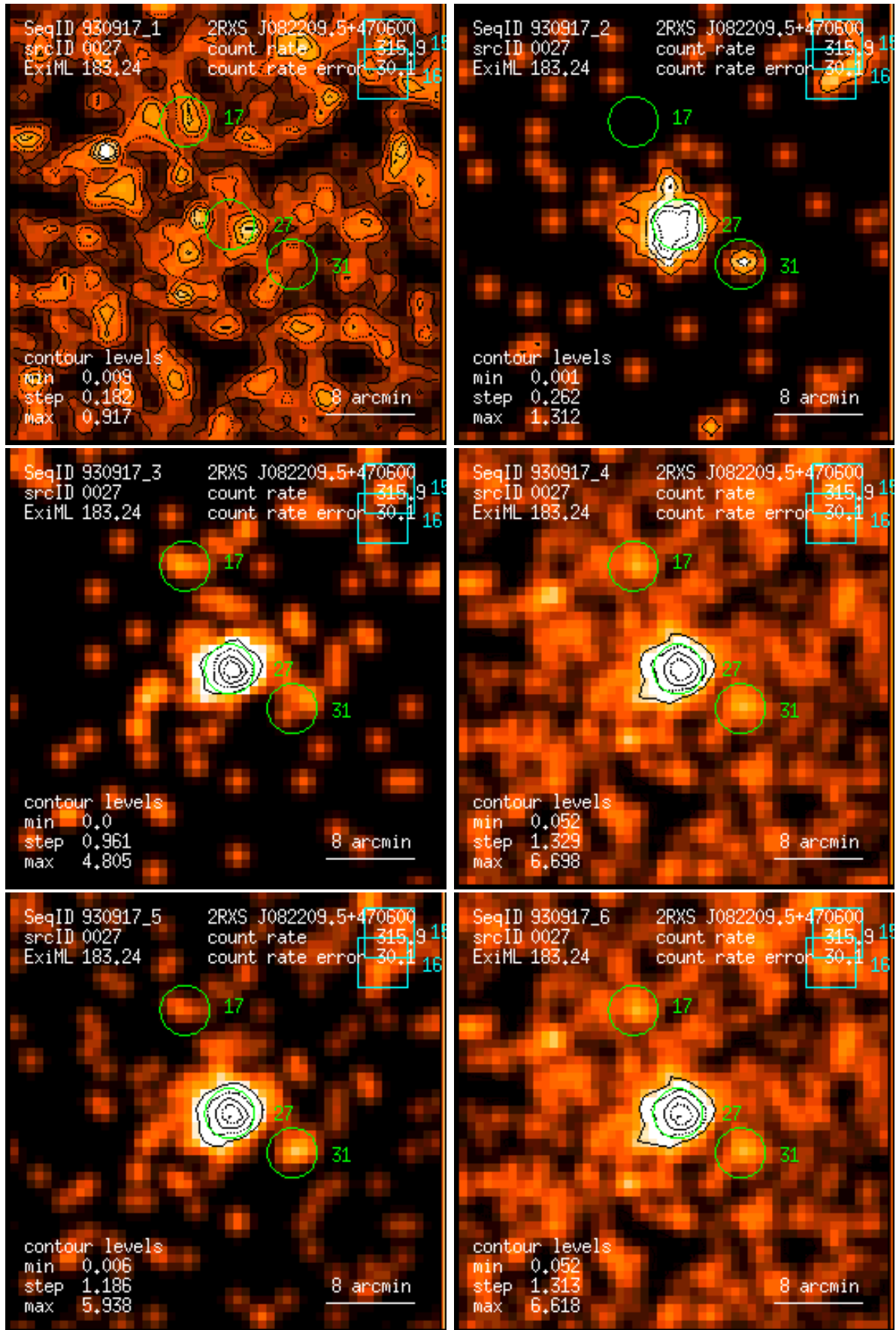
Figure 27: RASS 930917: detection 0027: band rate images, Gaussian filter: (1) PSPC channels 11 – 41, (2) 52 – 90, (3) 91 – 201, (4) 11 – 235, (5) 52 – 201, (6) 11 – 201. Broad band rates in counts/ks. Band rate contour levels in counts/ks/arcmin 2 .
