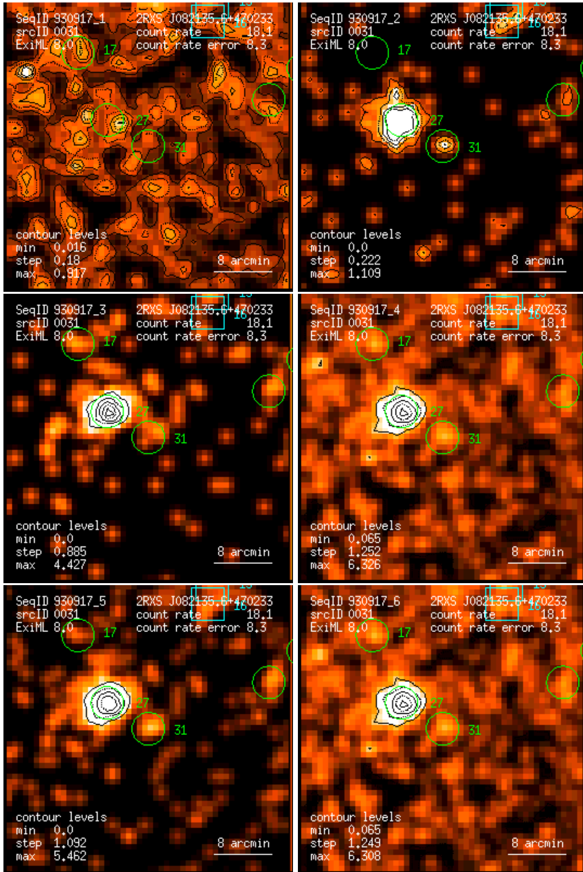
Figure 31: RASS 930917: detection 0031: band rate images, Gaussian filter: (1) PSPC channels 11 – 41, (2) 52 – 90, (3) 91 – 201, (4) 11 – 235, (5) 52 – 201, (6) 11 – 201. Broad band rates in counts/ks. Band rate contour levels in counts/ks/arcmin 2 .
