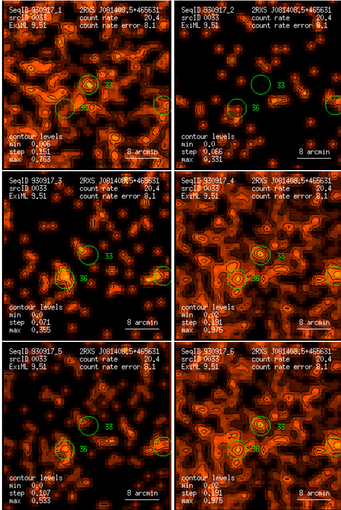
Figure 33: RASS 930917: detection 0033: band rate images, Gaussian filter: (1) PSPC channels 11 – 41, (2) 52 – 90, (3) 91 – 201, (4) 11 – 235, (5) 52 – 201, (6) 11 – 201. Broad band rates in counts/ks. Band rate contour levels in counts/ks/arcmin 2 .
