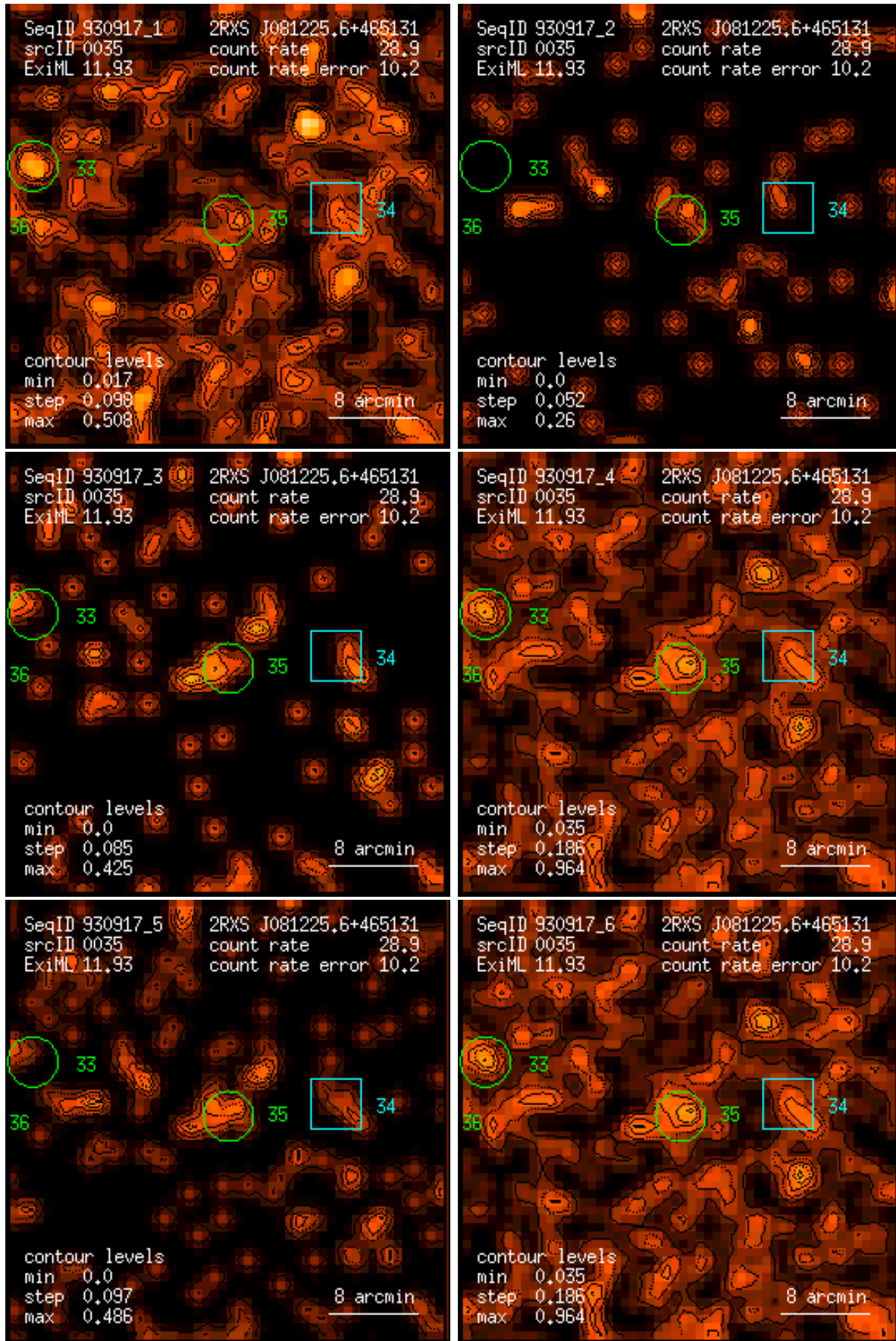
Figure 35: RASS 930917: detection 0035: band rate images, Gaussian filter: (1) PSPC channels 11 – 41, (2) 52 – 90, (3) 91 – 201, (4) 11 – 235, (5) 52 – 201, (6) 11 – 201. Broad band rates in counts/ks. Band rate contour levels in counts/ks/arcmin 2 .
