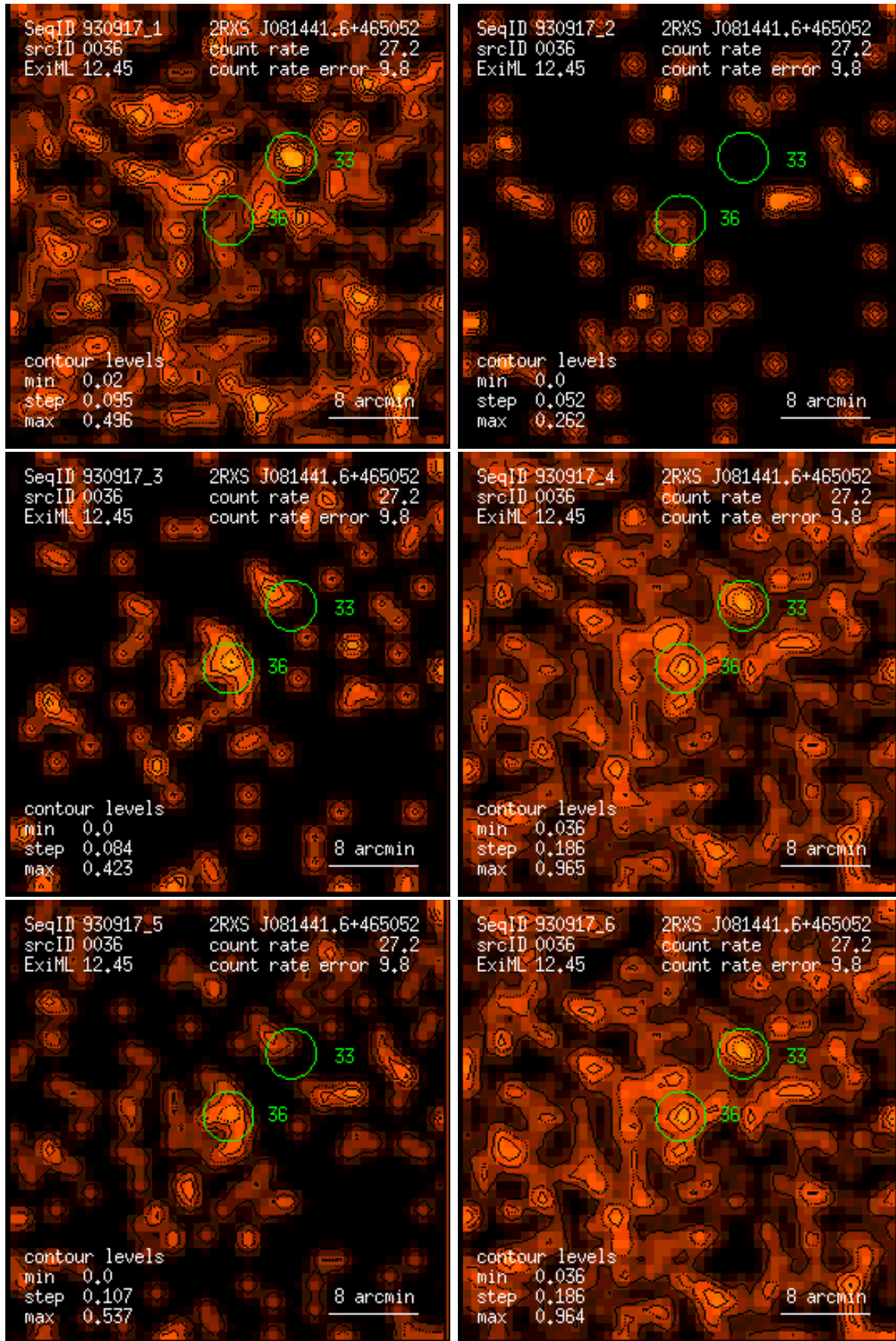
Figure 36: RASS 930917: detection 0036: band rate images, Gaussian filter: (1) PSPC channels 11 – 41, (2) 52 – 90, (3) 91 – 201, (4) 11 – 235, (5) 52 – 201, (6) 11 – 201. Broad band rates in counts/ks. Band rate contour levels in counts/ks/arcmin 2 .
