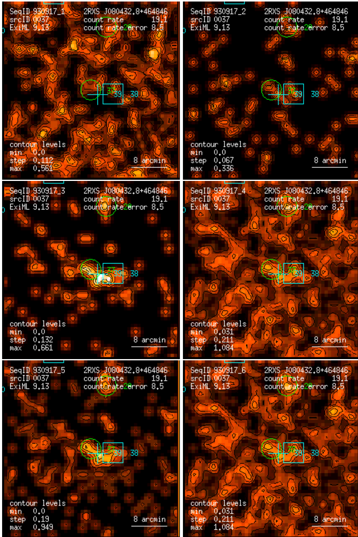
Figure 37: RASS 930917: detection 0037: band rate images, Gaussian filter: (1) PSPC channels 11 – 41, (2) 52 – 90, (3) 91 – 201, (4) 11 – 235, (5) 52 – 201, (6) 11 – 201. Broad band rates in counts/ks. Band rate contour levels in counts/ks/arcmin 2 .
