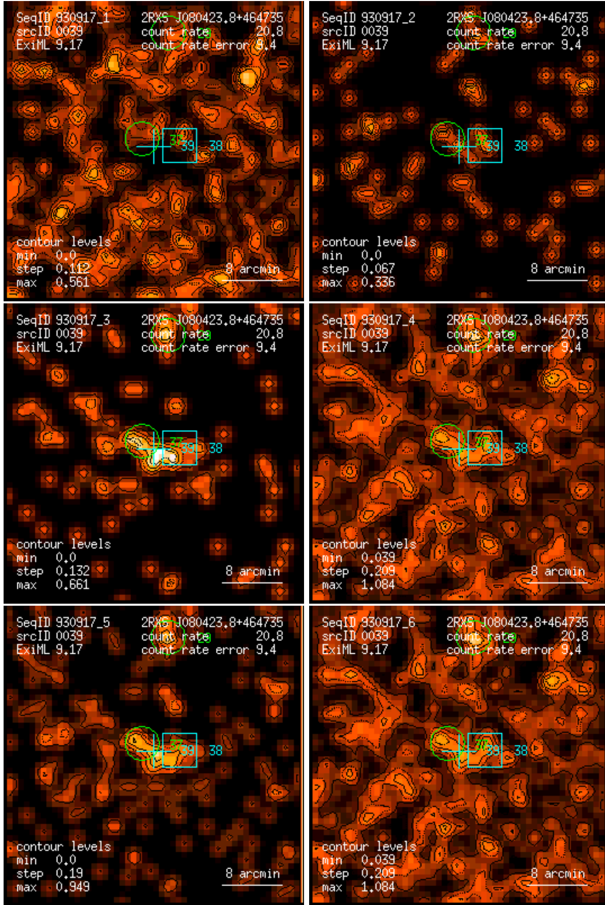
Figure 39: RASS 930917: detection 0039: band rate images, Gaussian filter: (1) PSPC channels 11 – 41, (2) 52 – 90, (3) 91 – 201, (4) 11 – 235, (5) 52 – 201, (6) 11 – 201. Broad band rates in counts/ks. Band rate contour levels in counts/ks/arcmin 2 .
