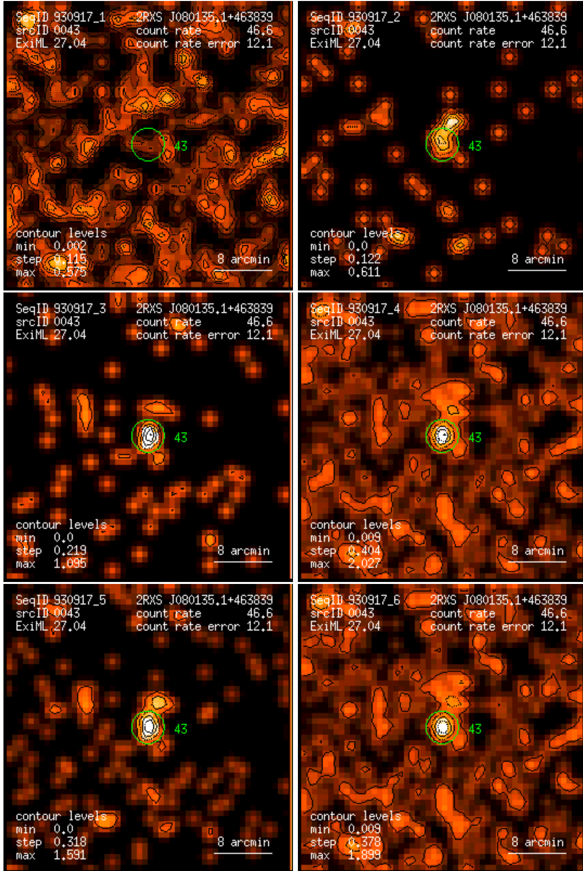
Figure 43: RASS 930917: detection 0043: band rate images, Gaussian filter: (1) PSPC channels 11 – 41, (2) 52 – 90, (3) 91 – 201, (4) 11 – 235, (5) 52 – 201, (6) 11 – 201. Broad band rates in counts/ks. Band rate contour levels in counts/ks/arcmin 2 .
