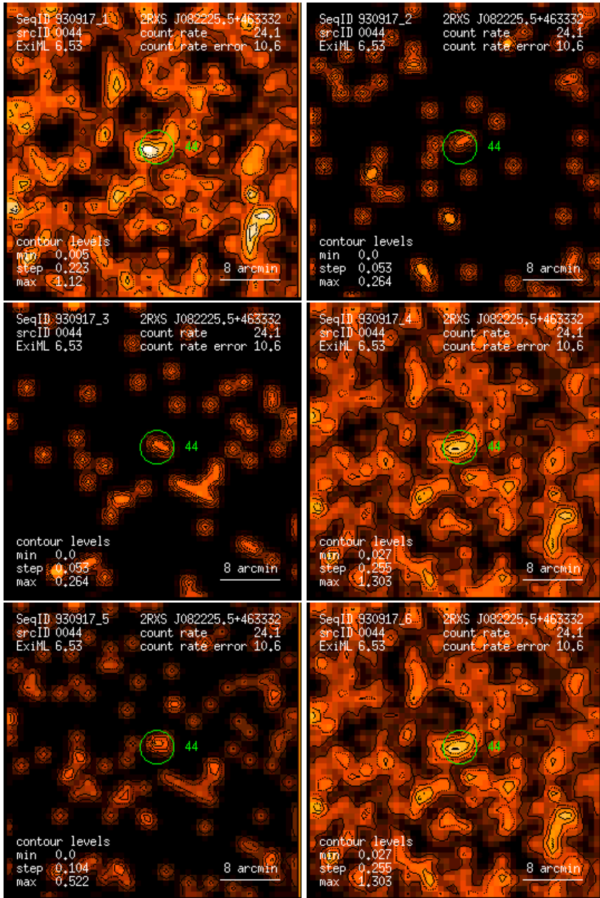
Figure 44: RASS 930917: detection 0044: band rate images, Gaussian filter: (1) PSPC channels 11 – 41, (2) 52 – 90, (3) 91 – 201, (4) 11 – 235, (5) 52 – 201, (6) 11 – 201. Broad band rates in counts/ks. Band rate contour levels in counts/ks/arcmin 2 .
