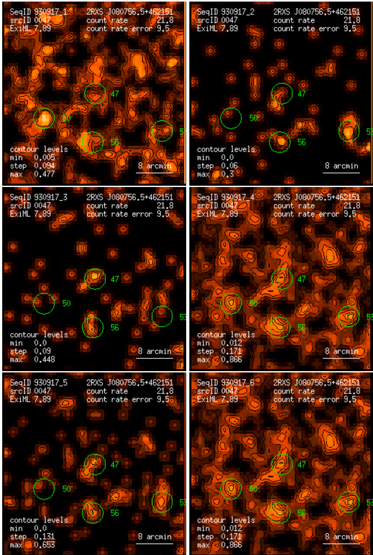
Figure 47: RASS 930917: detection 0047: band rate images, Gaussian filter: (1) PSPC channels 11 – 41, (2) 52 – 90, (3) 91 – 201, (4) 11 – 235, (5) 52 – 201, (6) 11 – 201. Broad band rates in counts/ks. Band rate contour levels in counts/ks/arcmin 2 .
