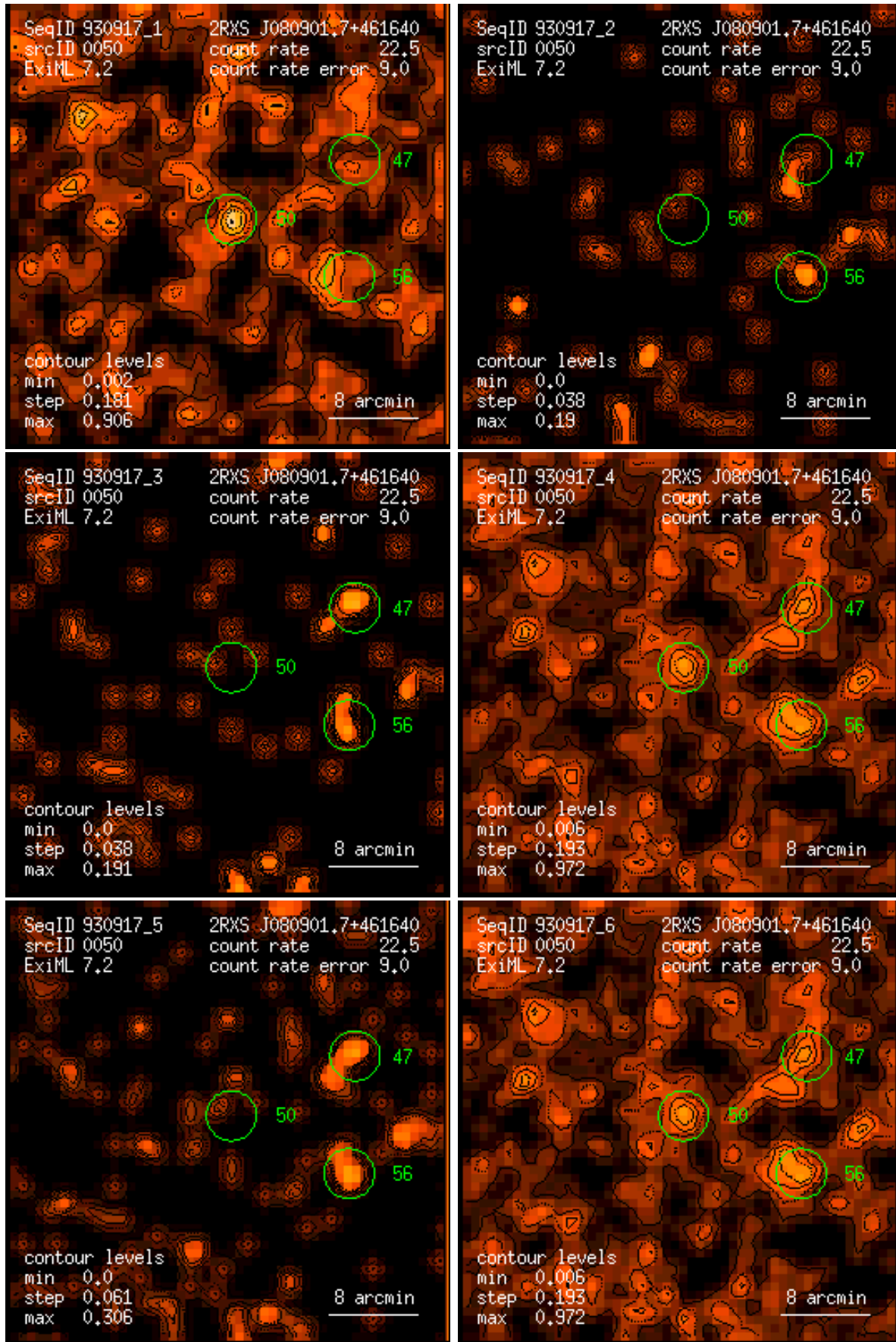
Figure 50: RASS 930917: detection 0050: band rate images, Gaussian filter: (1) PSPC channels 11 – 41, (2) 52 – 90, (3) 91 – 201, (4) 11 – 235, (5) 52 – 201, (6) 11 – 201. Broad band rates in counts/ks. Band rate contour levels in counts/ks/arcmin 2 .
