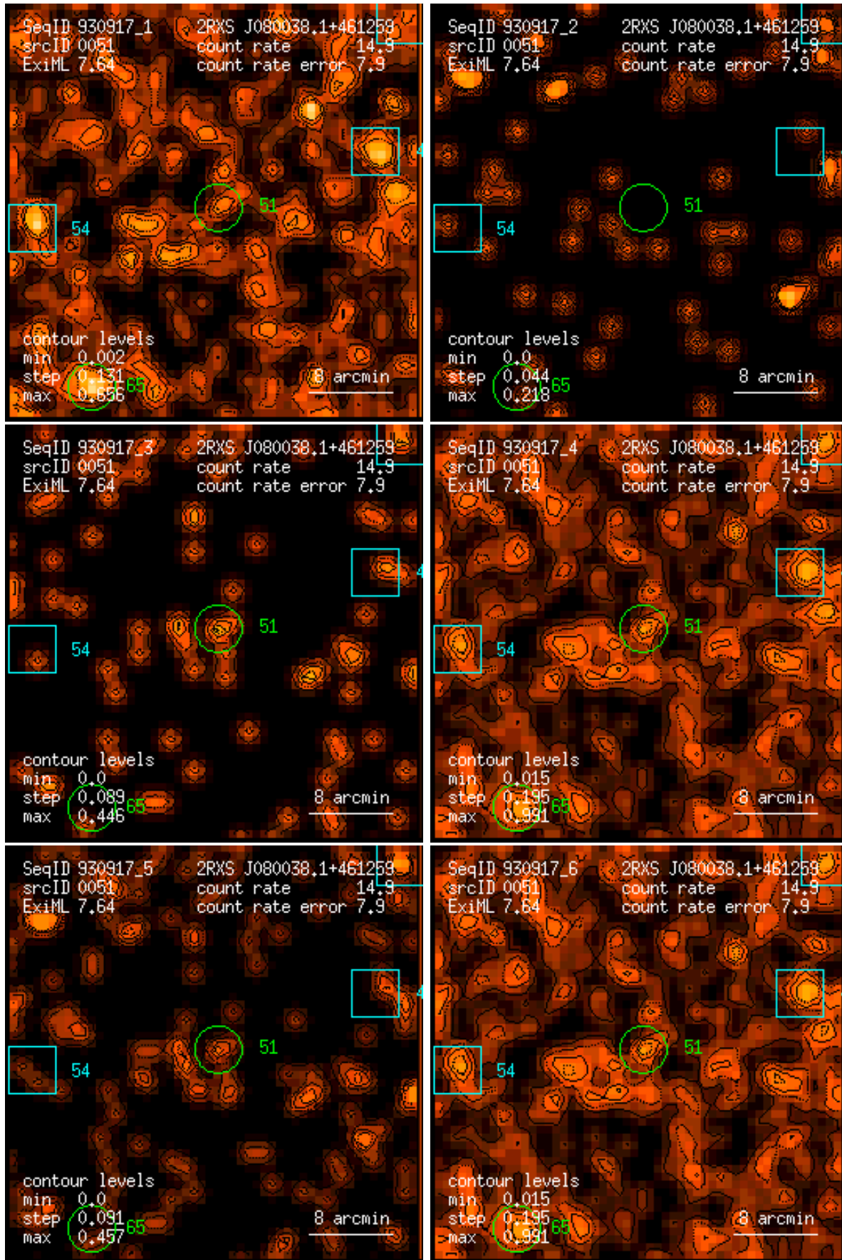
Figure 51: RASS 930917: detection 0051: band rate images, Gaussian filter: (1) PSPC channels 11 – 41, (2) 52 – 90, (3) 91 – 201, (4) 11 – 235, (5) 52 – 201, (6) 11 – 201. Broad band rates in counts/ks. Band rate contour levels in counts/ks/arcmin 2 .
