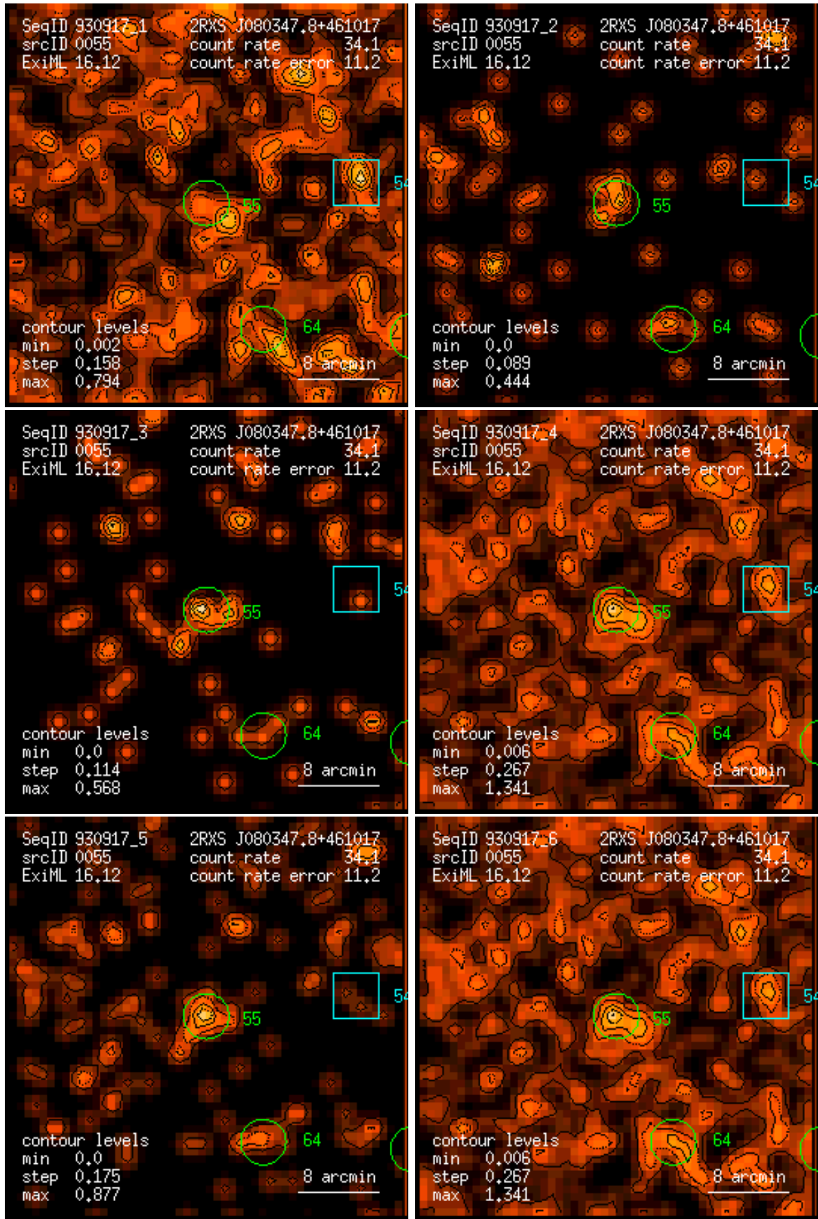
Figure 55: RASS 930917: detection 0055: band rate images, Gaussian filter: (1) PSPC channels 11 – 41, (2) 52 – 90, (3) 91 – 201, (4) 11 – 235, (5) 52 – 201, (6) 11 – 201. Broad band rates in counts/ks. Band rate contour levels in counts/ks/arcmin 2 .
