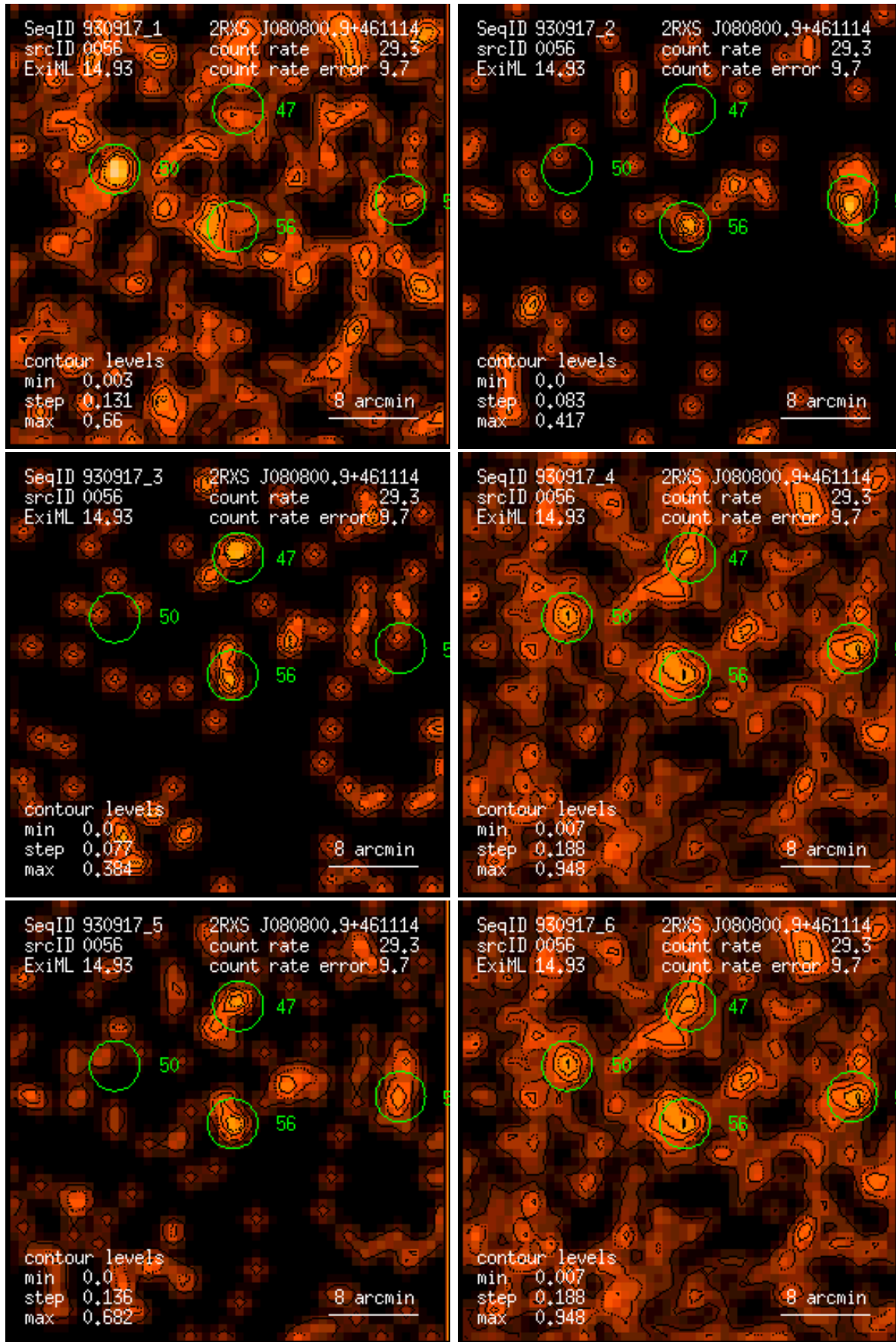
Figure 56: RASS 930917: detection 0056: band rate images, Gaussian filter: (1) PSPC channels 11 – 41, (2) 52 – 90, (3) 91 – 201, (4) 11 – 235, (5) 52 – 201, (6) 11 – 201. Broad band rates in counts/ks. Band rate contour levels in counts/ks/arcmin 2 .
