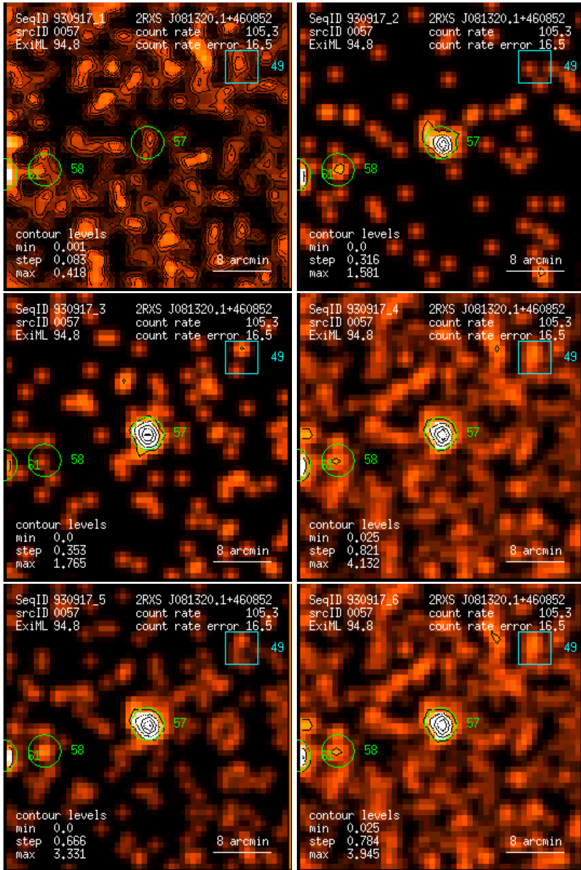
Figure 57: RASS 930917: detection 0057: band rate images, Gaussian filter: (1) PSPC channels 11 – 41, (2) 52 – 90, (3) 91 – 201, (4) 11 – 235, (5) 52 – 201, (6) 11 – 201. Broad band rates in counts/ks. Band rate contour levels in counts/ks/arcmin 2 .
