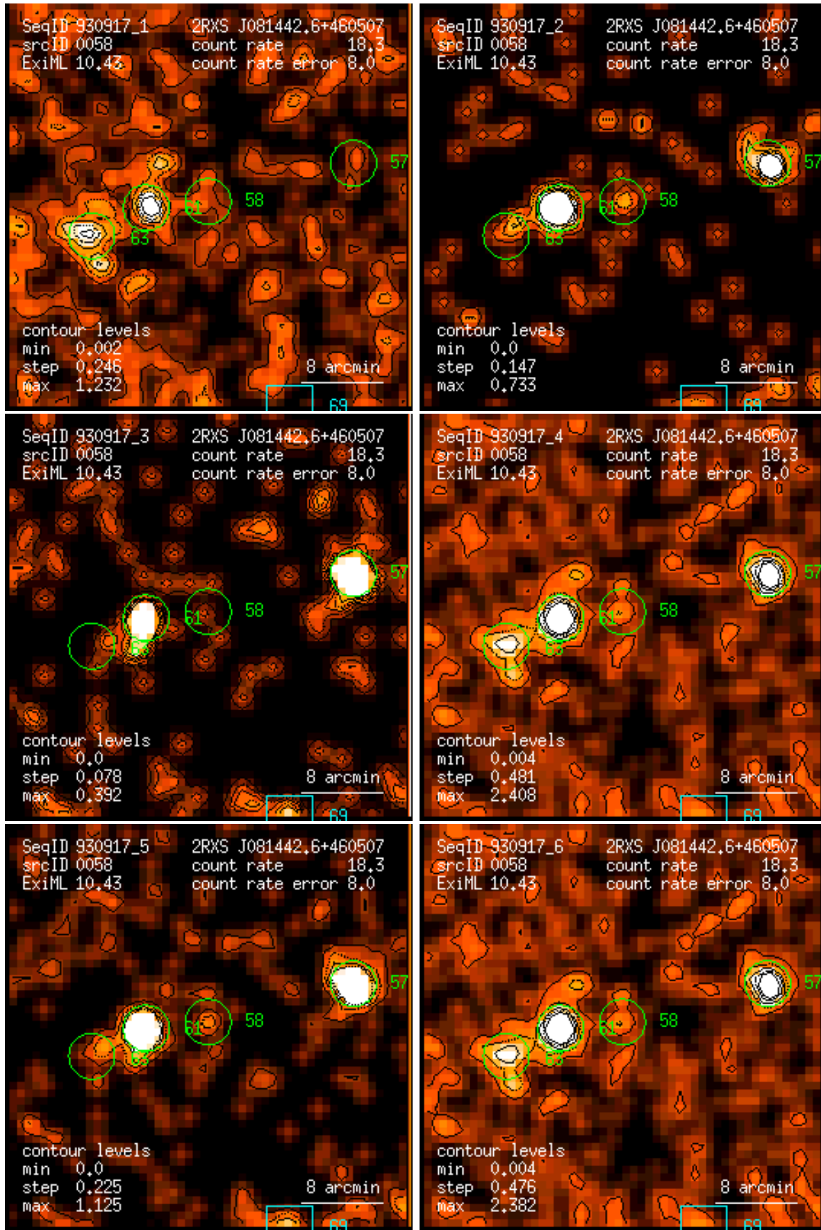
Figure 58: RASS 930917: detection 0058: band rate images, Gaussian filter: (1) PSPC channels 11 – 41, (2) 52 – 90, (3) 91 – 201, (4) 11 – 235, (5) 52 – 201, (6) 11 – 201. Broad band rates in counts/ks. Band rate contour levels in counts/ks/arcmin 2 .
