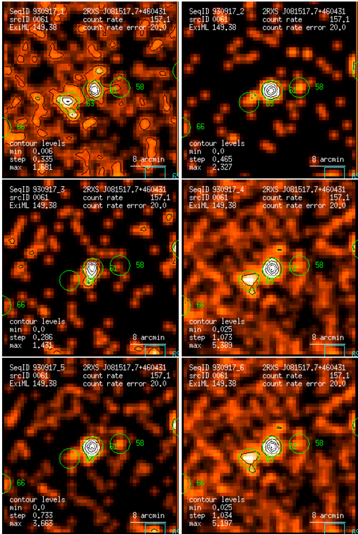
Figure 61: RASS 930917: detection 0061: band rate images, Gaussian filter: (1) PSPC channels 11 – 41, (2) 52 – 90, (3) 91 – 201, (4) 11 – 235, (5) 52 – 201, (6) 11 – 201. Broad band rates in counts/ks. Band rate contour levels in counts/ks/arcmin 2 .
