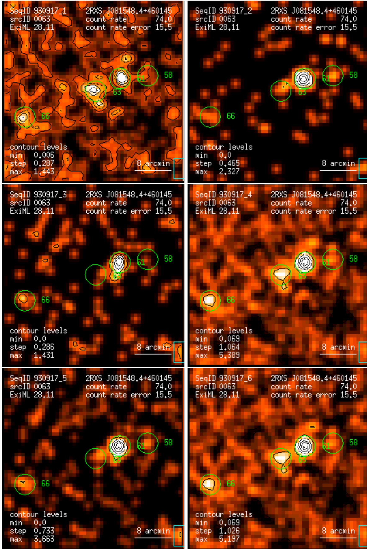
Figure 63: RASS 930917: detection 0063: band rate images, Gaussian filter: (1) PSPC channels 11 – 41, (2) 52 – 90, (3) 91 – 201, (4) 11 – 235, (5) 52 – 201, (6) 11 – 201. Broad band rates in counts/ks. Band rate contour levels in counts/ks/arcmin 2 .
