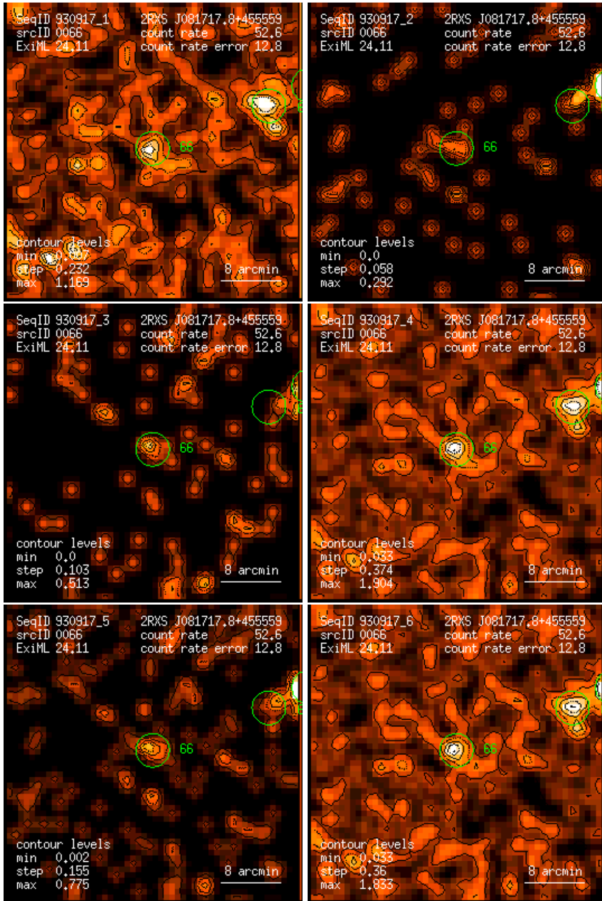
Figure 66: RASS 930917: detection 0066: band rate images, Gaussian filter: (1) PSPC channels 11 – 41, (2) 52 – 90, (3) 91 – 201, (4) 11 – 235, (5) 52 – 201, (6) 11 – 201. Broad band rates in counts/ks. Band rate contour levels in counts/ks/arcmin 2 .
