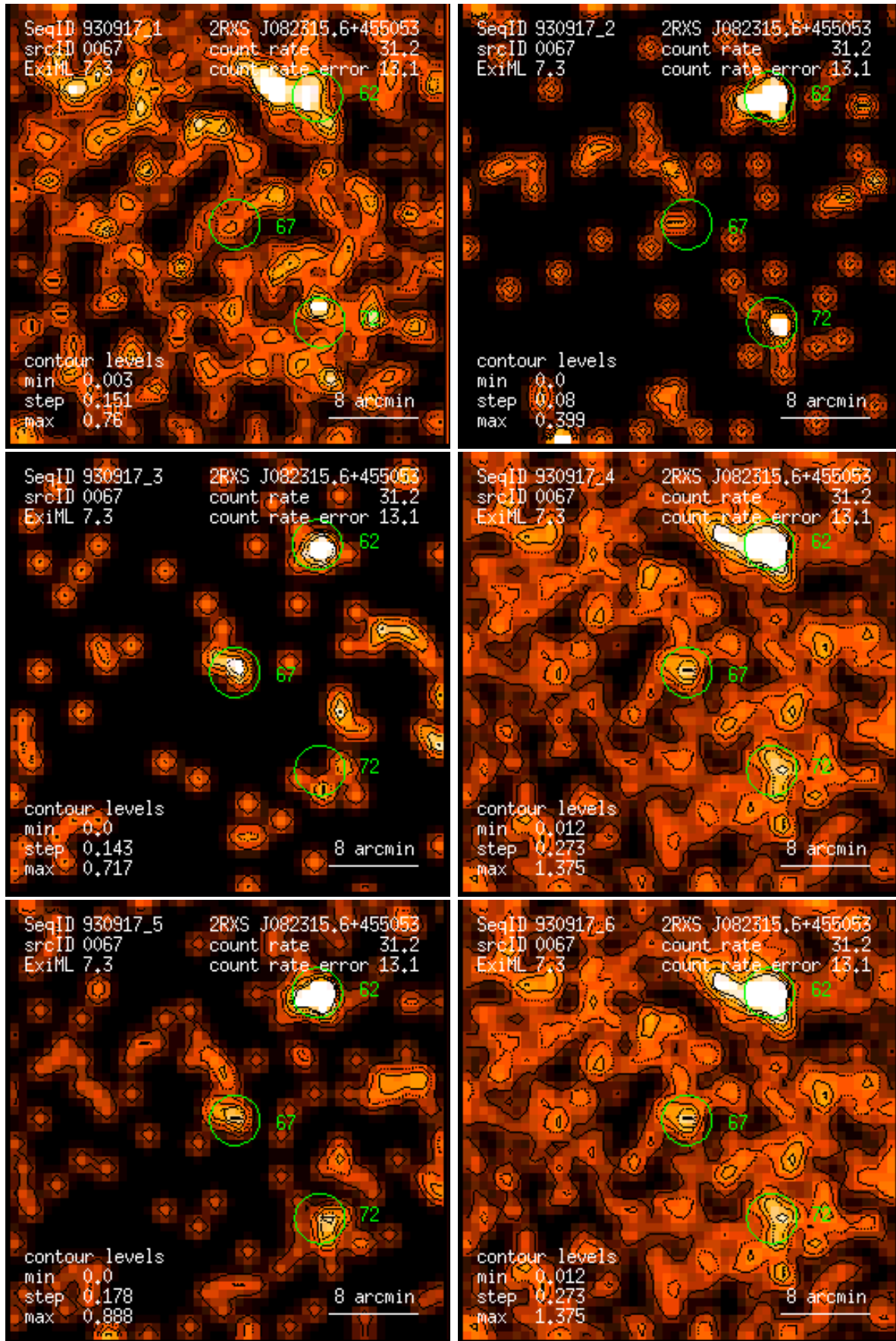
Figure 67: RASS 930917: detection 0067: band rate images, Gaussian filter: (1) PSPC channels 11 – 41, (2) 52 – 90, (3) 91 – 201, (4) 11 – 235, (5) 52 – 201, (6) 11 – 201. Broad band rates in counts/ks. Band rate contour levels in counts/ks/arcmin 2 .
