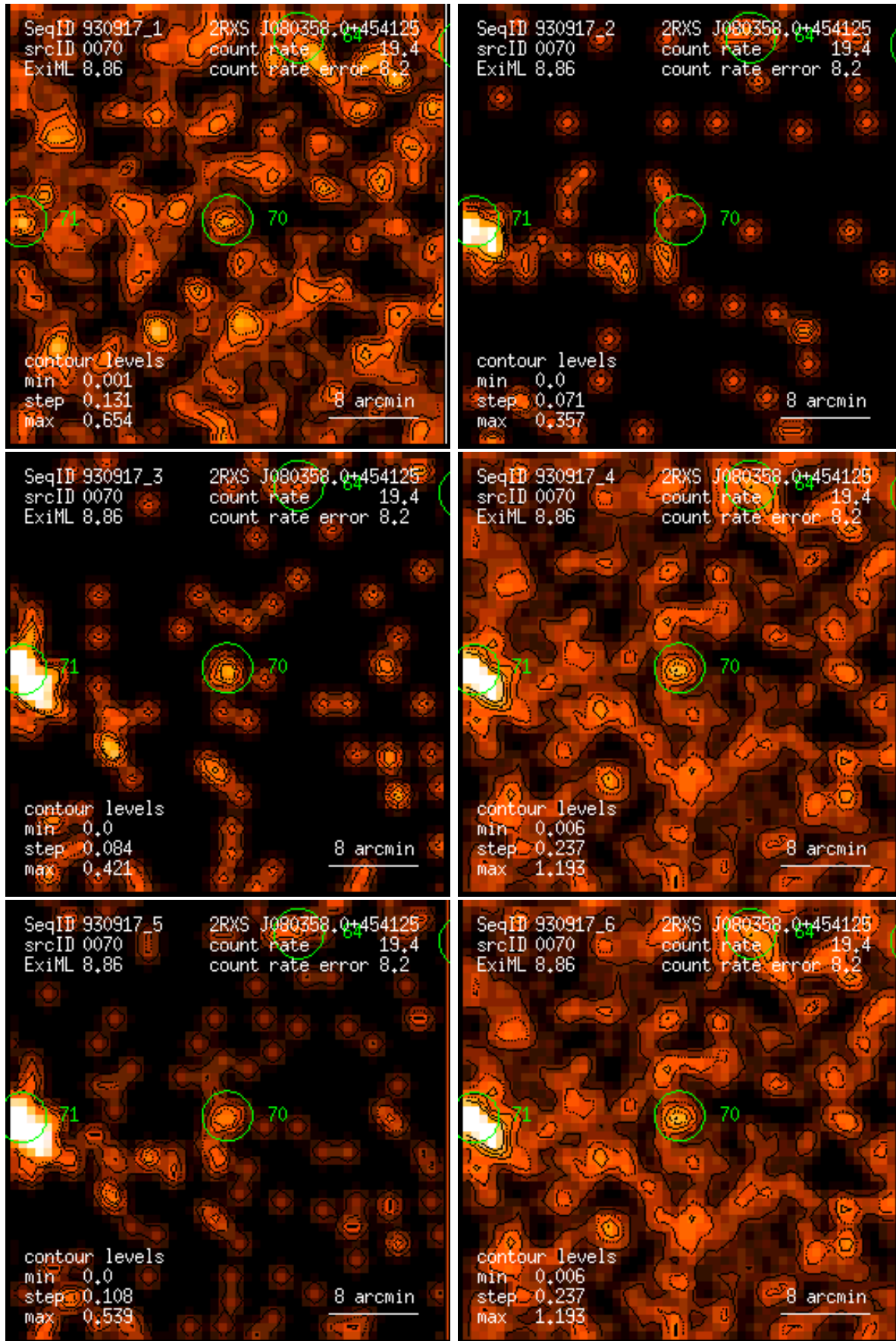
Figure 70: RASS 930917: detection 0070: band rate images, Gaussian filter: (1) PSPC channels 11 – 41, (2) 52 – 90, (3) 91 – 201, (4) 11 – 235, (5) 52 – 201, (6) 11 – 201. Broad band rates in counts/ks. Band rate contour levels in counts/ks/arcmin 2 .
