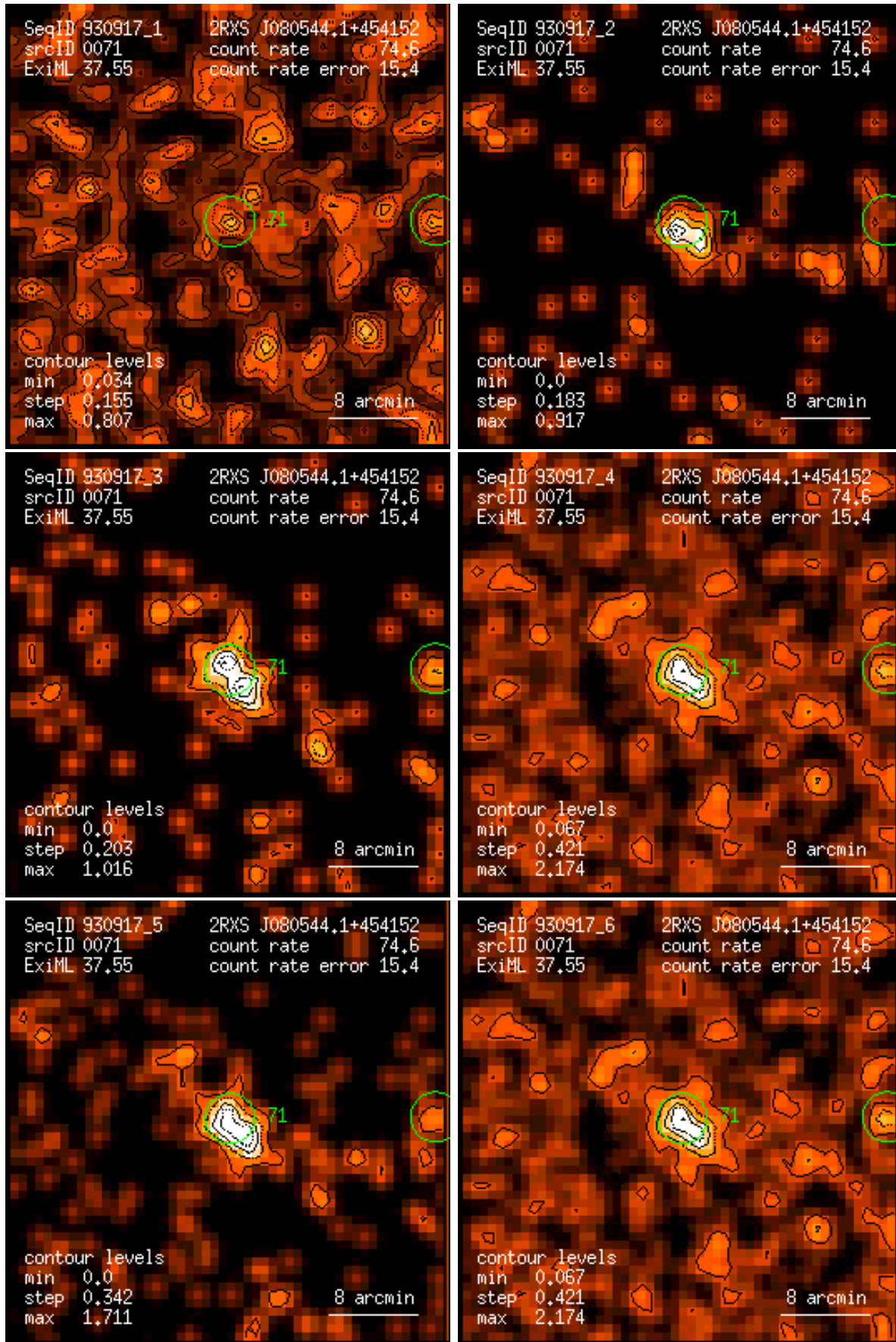
Figure 71: RASS 930917: detection 0071: band rate images, Gaussian filter: (1) PSPC channels 11 – 41, (2) 52 – 90, (3) 91 – 201, (4) 11 – 235, (5) 52 – 201, (6) 11 – 201. Broad band rates in counts/ks. Band rate contour levels in counts/ks/arcmin 2 .
