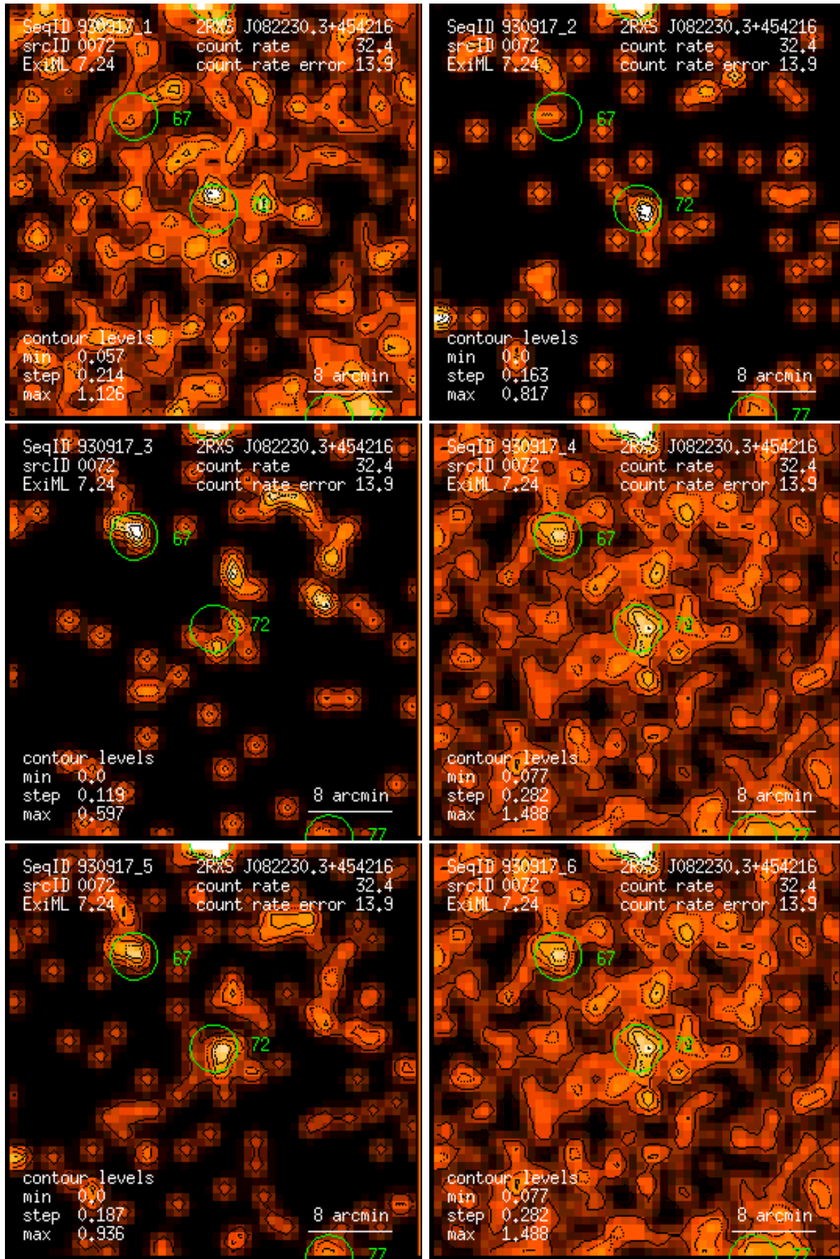
Figure 72: RASS 930917: detection 0072: band rate images, Gaussian filter: (1) PSPC channels 11 – 41, (2) 52 – 90, (3) 91 – 201, (4) 11 – 235, (5) 52 – 201, (6) 11 – 201. Broad band rates in counts/ks. Band rate contour levels in counts/ks/arcmin 2 .
