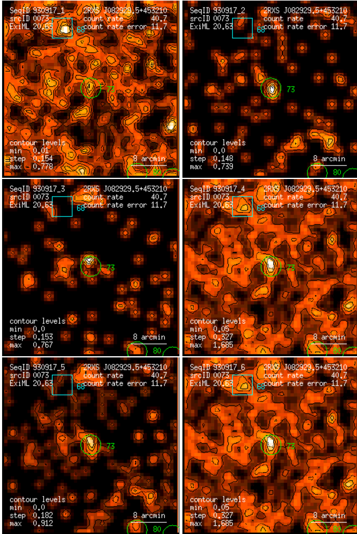
Figure 73: RASS 930917: detection 0073: band rate images, Gaussian filter: (1) PSPC channels 11 – 41, (2) 52 – 90, (3) 91 – 201, (4) 11 – 235, (5) 52 – 201, (6) 11 – 201. Broad band rates in counts/ks. Band rate contour levels in counts/ks/arcmin 2 .
