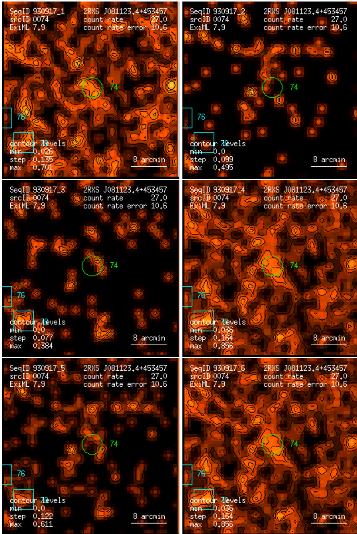
Figure 74: RASS 930917: detection 0074: band rate images, Gaussian filter: (1) PSPC channels 11 – 41, (2) 52 – 90, (3) 91 – 201, (4) 11 – 235, (5) 52 – 201, (6) 11 – 201. Broad band rates in counts/ks. Band rate contour levels in counts/ks/arcmin 2 .
