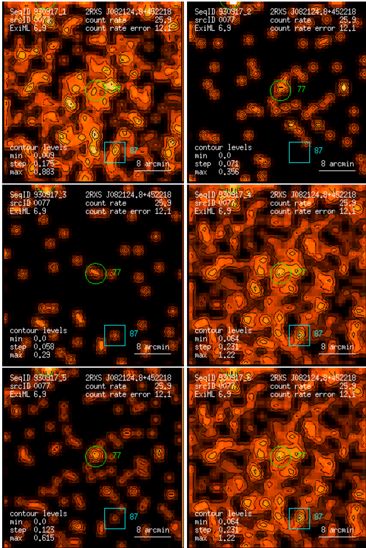
Figure 77: RASS 930917: detection 0077: band rate images, Gaussian filter: (1) PSPC channels 11 – 41, (2) 52 – 90, (3) 91 – 201, (4) 11 – 235, (5) 52 – 201, (6) 11 – 201. Broad band rates in counts/ks. Band rate contour levels in counts/ks/arcmin 2 .
