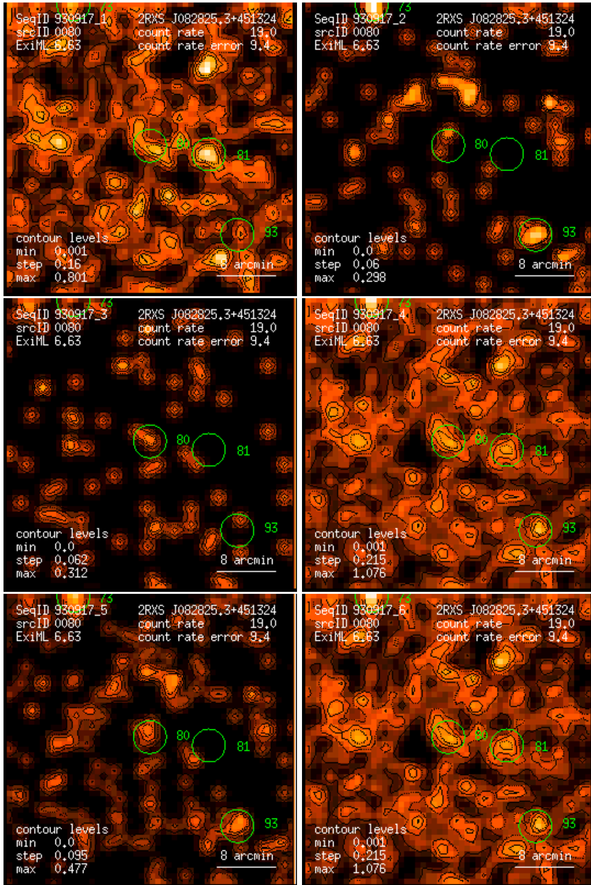
Figure 80: RASS 930917: detection 0080: band rate images, Gaussian filter: (1) PSPC channels 11 – 41, (2) 52 – 90, (3) 91 – 201, (4) 11 – 235, (5) 52 – 201, (6) 11 – 201. Broad band rates in counts/ks. Band rate contour levels in counts/ks/arcmin 2 .
