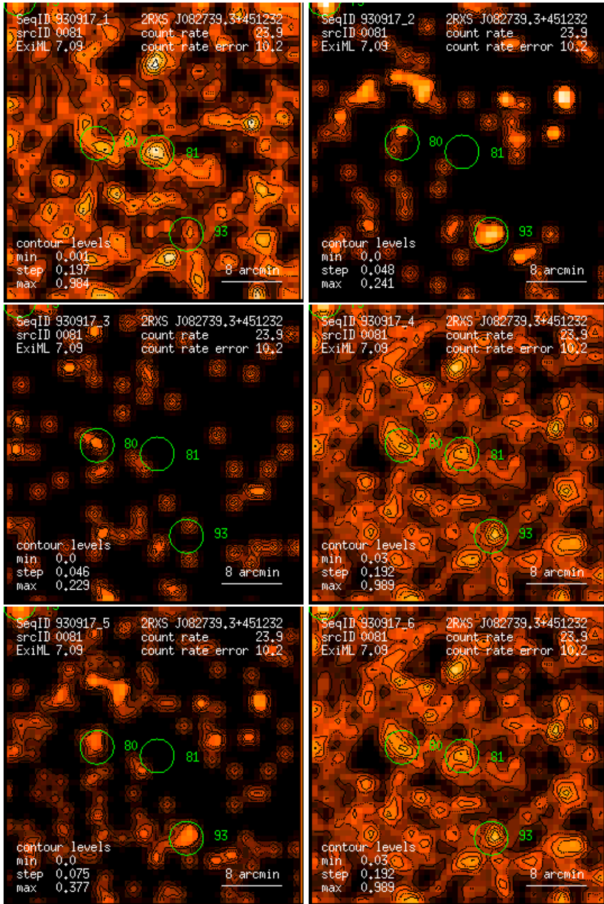
Figure 81: RASS 930917: detection 0081: band rate images, Gaussian filter: (1) PSPC channels 11 – 41, (2) 52 – 90, (3) 91 – 201, (4) 11 – 235, (5) 52 – 201, (6) 11 – 201. Broad band rates in counts/ks. Band rate contour levels in counts/ks/arcmin 2 .
