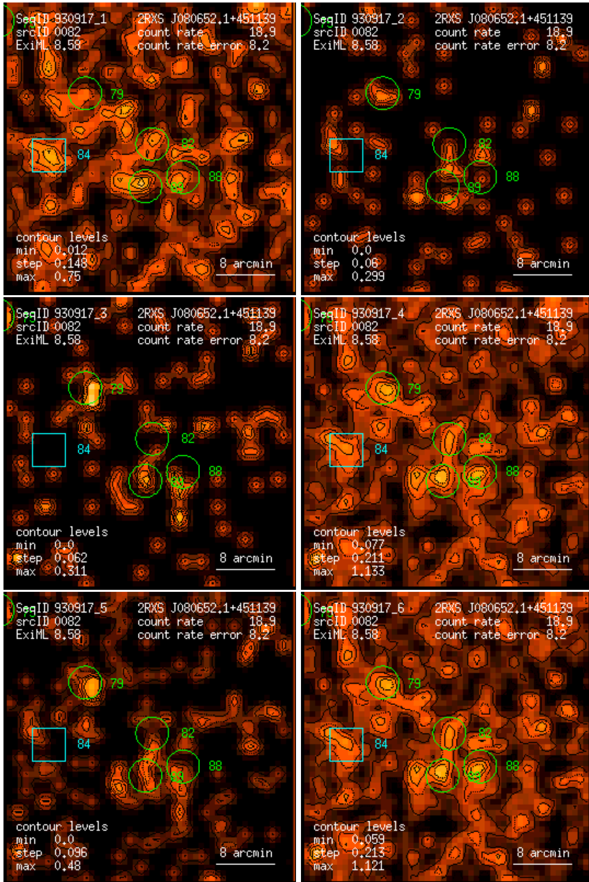
Figure 82: RASS 930917: detection 0082: band rate images, Gaussian filter: (1) PSPC channels 11 – 41, (2) 52 – 90, (3) 91 – 201, (4) 11 – 235, (5) 52 – 201, (6) 11 – 201. Broad band rates in counts/ks. Band rate contour levels in counts/ks/arcmin 2 .
