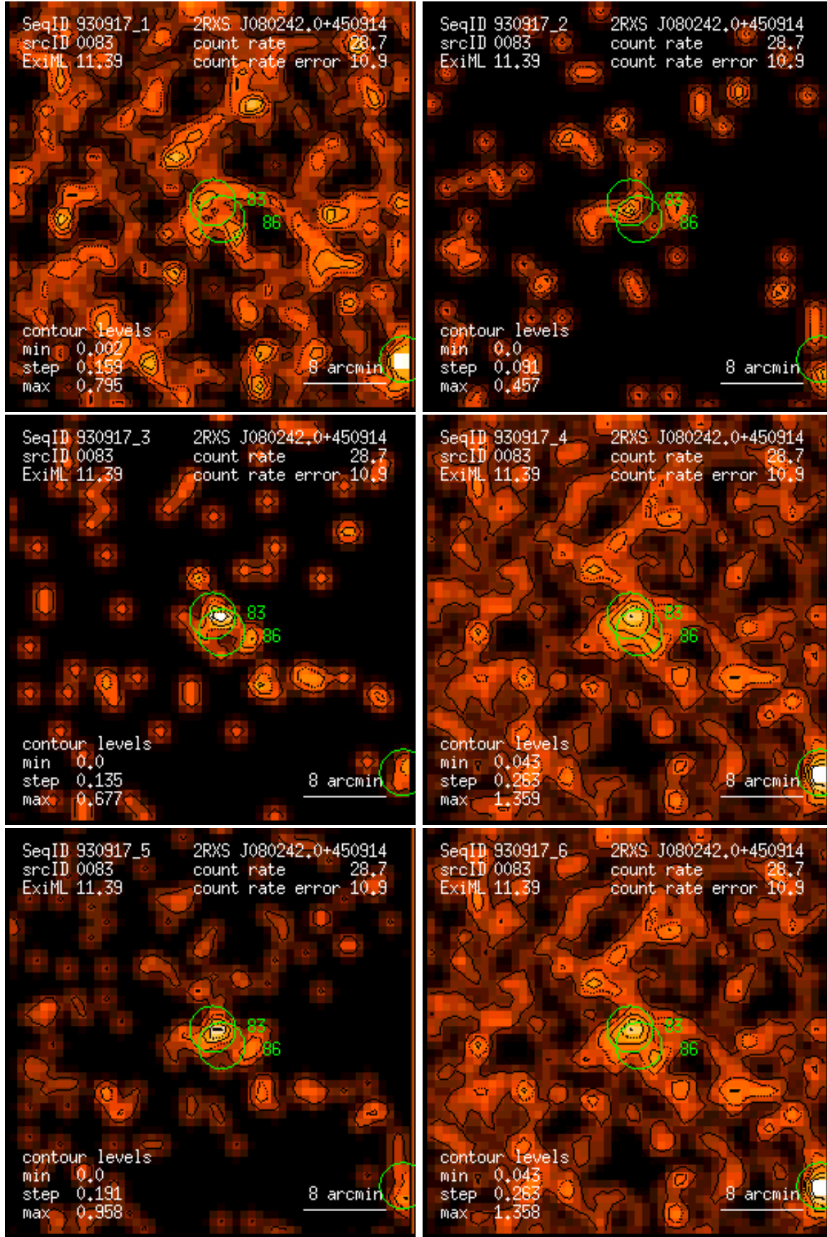
Figure 83: RASS 930917: detection 0083: band rate images, Gaussian filter: (1) PSPC channels 11 – 41, (2) 52 – 90, (3) 91 – 201, (4) 11 – 235, (5) 52 – 201, (6) 11 – 201. Broad band rates in counts/ks. Band rate contour levels in counts/ks/arcmin 2 .
