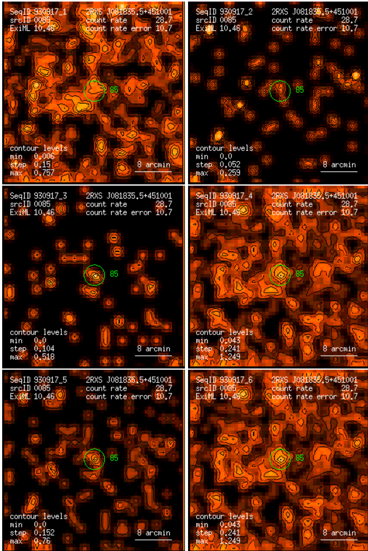
Figure 85: RASS 930917: detection 0085: band rate images, Gaussian filter: (1) PSPC channels 11 – 41, (2) 52 – 90, (3) 91 – 201, (4) 11 – 235, (5) 52 – 201, (6) 11 – 201. Broad band rates in counts/ks. Band rate contour levels in counts/ks/arcmin 2 .
