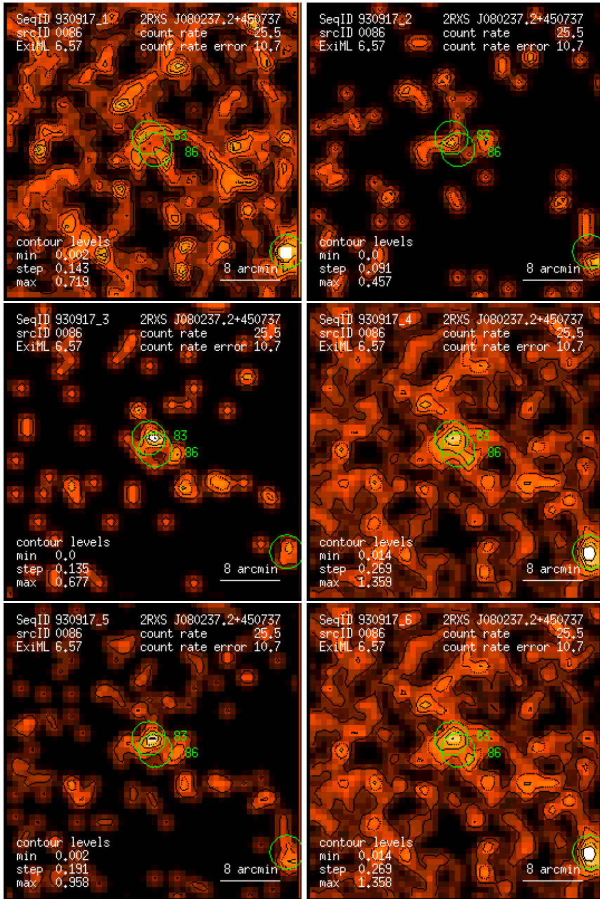
Figure 86: RASS 930917: detection 0086: band rate images, Gaussian filter: (1) PSPC channels 11 – 41, (2) 52 – 90, (3) 91 – 201, (4) 11 – 235, (5) 52 – 201, (6) 11 – 201. Broad band rates in counts/ks. Band rate contour levels in counts/ks/arcmin 2 .
