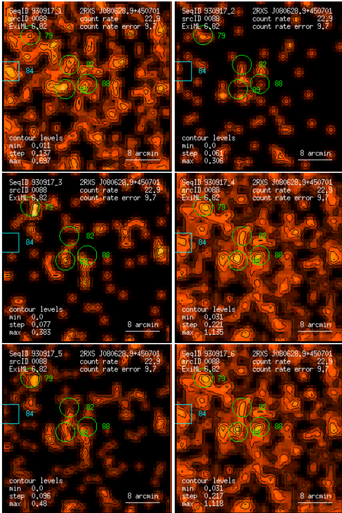
Figure 88: RASS 930917: detection 0088: band rate images, Gaussian filter: (1) PSPC channels 11 – 41, (2) 52 – 90, (3) 91 – 201, (4) 11 – 235, (5) 52 – 201, (6) 11 – 201. Broad band rates in counts/ks. Band rate contour levels in counts/ks/arcmin 2 .
