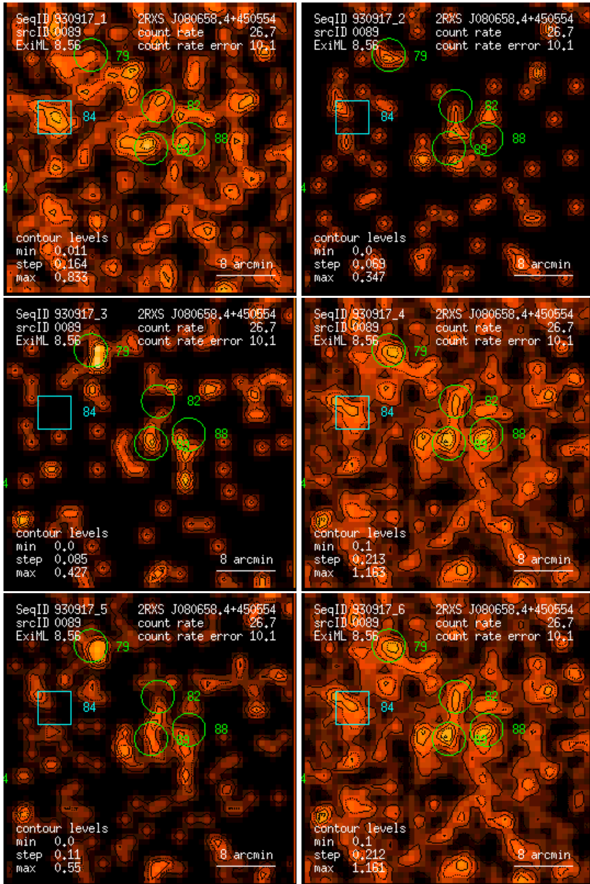
Figure 89: RASS 930917: detection 0089: band rate images, Gaussian filter: (1) PSPC channels 11 – 41, (2) 52 – 90, (3) 91 – 201, (4) 11 – 235, (5) 52 – 201, (6) 11 – 201. Broad band rates in counts/ks. Band rate contour levels in counts/ks/arcmin 2 .
