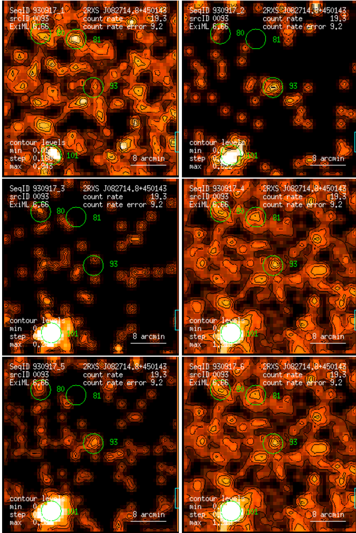
Figure 93: RASS 930917: detection 0093: band rate images, Gaussian filter: (1) PSPC channels 11 – 41, (2) 52 – 90, (3) 91 – 201, (4) 11 – 235, (5) 52 – 201, (6) 11 – 201. Broad band rates in counts/ks. Band rate contour levels in counts/ks/arcmin 2 .
