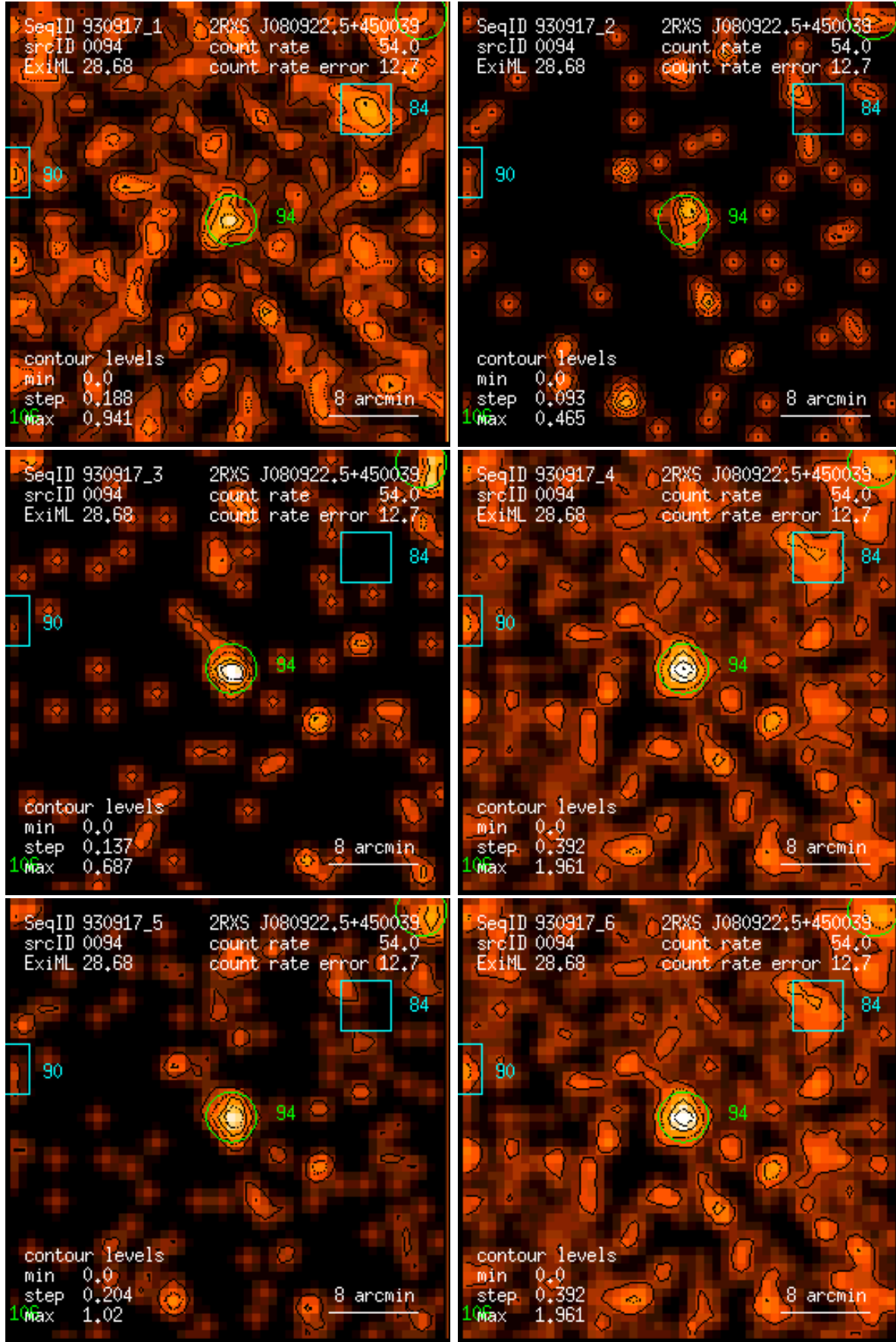
Figure 94: RASS 930917: detection 0094: band rate images, Gaussian filter: (1) PSPC channels 11 – 41, (2) 52 – 90, (3) 91 – 201, (4) 11 – 235, (5) 52 – 201, (6) 11 – 201. Broad band rates in counts/ks. Band rate contour levels in counts/ks/arcmin 2 .
