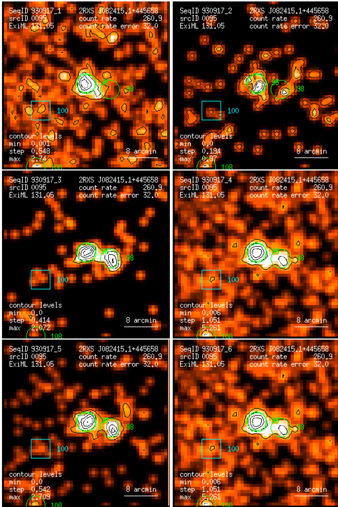
Figure 95: RASS 930917: detection 0095: band rate images, Gaussian filter: (1) PSPC channels 11 – 41, (2) 52 – 90, (3) 91 – 201, (4) 11 – 235, (5) 52 – 201, (6) 11 – 201. Broad band rates in counts/ks. Band rate contour levels in counts/ks/arcmin 2 .
