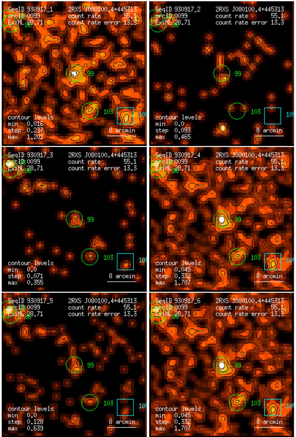
Figure 99: RASS 930917: detection 0099: band rate images, Gaussian filter: (1) PSPC channels 11 – 41, (2) 52 – 90, (3) 91 – 201, (4) 11 – 235, (5) 52 – 201, (6) 11 – 201. Broad band rates in counts/ks. Band rate contour levels in counts/ks/arcmin 2 .
